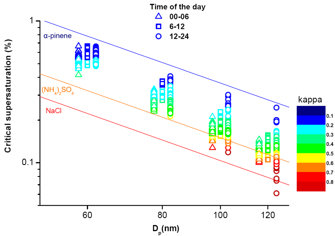
Fig. 11. Measured critical supersaturations of 60, 80, 100 and 120 nm diameter particles during different times of the day on 28 and 30 August, 2012. The color scale indicates different values of the particle hygroscopicity parameter, \kappa . Also, theoretical curves for \alpha -pinene, ammonium sulfate and sodium chloride.
