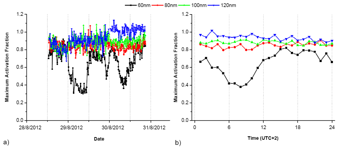
Fig. 10. a) Maximum activation fraction of 60,80, 100 and 120 nm particles between 28 and 30 August, 2012. b) Diurnal cycle of the maximum activated fraction for the same period.
