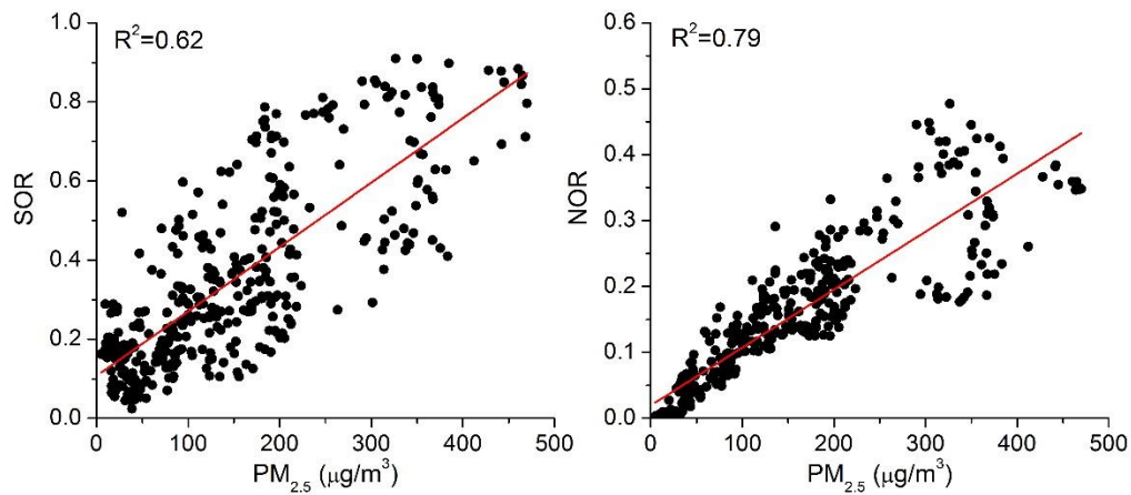
Fig.2 Relationship between PM 2.5 and SOR, NOR
