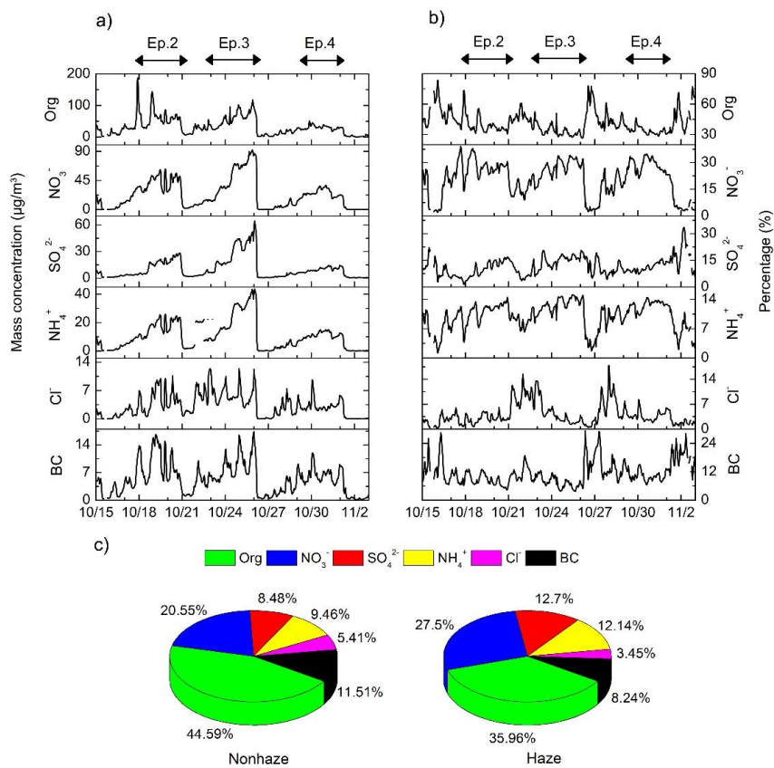
Fig. 6 a) temporal variation of the mass concentration of each aerosol species in \text{PM}_{10} , b) temporal variation of the mass fraction of each aerosol species in \text{PM}_{10} , c) mass fraction of each aerosol species in \text{PM}_{10} during non-haze and haze episodes from 15 October to 2 November 2014.
