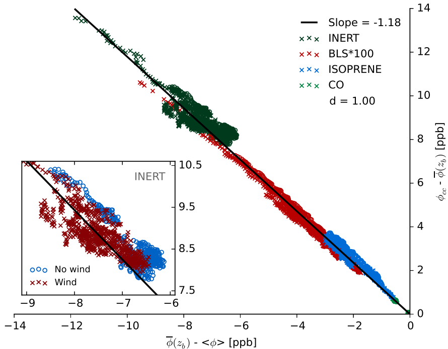
Figure 7. Parameterization for \bar{\phi}_{cc} - \bar{\phi}(z_b) as a function of \bar{\phi}(z_b) - \langle \phi \rangle proposed by Ouwersloot et al. (2013). Here, \phi represents the 24 transported species (note that only INERT, BLS, isoprene and CO are shown). Circles represent free convection situations, crosses indicate wind situations. The solid line represents a least square fit trough all data, which is forced through 0. d represents the index of agreement. The inset shows solely the INERT species for wind and no wind experiments.
