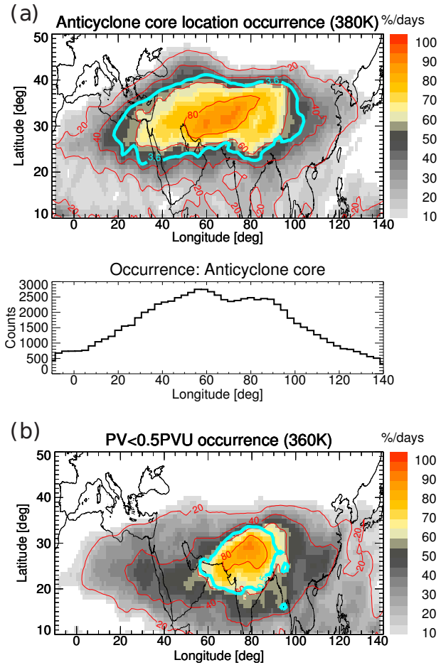
Fig. 113. (a) Occurrence frequency of the Asian monsoon anticyclone at 380 K (in percentage of days) for the period between 20 June and 20 August 2011, calculated from the area covered by PV values lower than the anticyclone transport barrier. Red contours show selected percentage values (20, 40, 60, 80%), the thick cyan contour shows the average PV value of the barrier in the average PV field (average over the period considered). The bottom panel shows the projection of anticyclone occurrence frequency onto the longitude axis (bin size 2.5^\circ ). (b) Occurrence frequency for PV values below 0.5 PVU at 360 K isentropic, for the same period (cyan contour shows 0.5 PVU in the average PV field).
