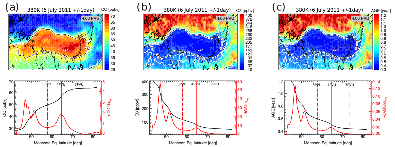
Fig. 111. (a) Map of CO from CLaMS on the 380 K isentropic, with the thick white contour showing the PV-value of maximum CO-gradient, the black contour showing the PV-value of maximum PV-gradient (thin white line shows 5 PVU), averaged between 5 and 7 July 2011 at 380 K. The bottom panel shows CO from CLaMS versus monsoon centered equivalent latitude (black), and the respective gradient (red). (b) Same for ozone from CLaMS, and (c) for mean age from CLaMS. (The PV values of the maximum gradient are given in the upper panels.)
