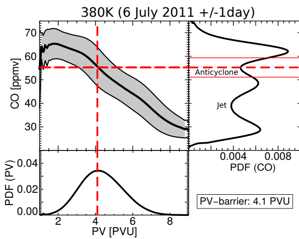
Fig. 115. Asian monsoon transport barrier at 380 K on 6 July 2011 from the CO mixing ratio PDF. The main panel (upper left) shows CLaMS CO (monsoon region average, 5–7 July time average) versus PV with one standard deviation as grey shading. The upper right panel shows the corresponding mixing ratio PDF with the monsoon transport barrier highlighted as red dashed line. The lower panel shows the PDF of PV-values around the barrier (between the thin red lines in the upper right panel). (See text for further details.)
