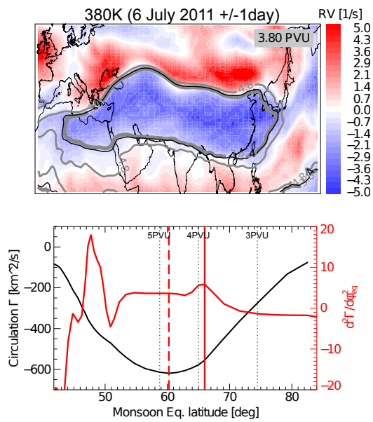
Fig. 17. Relative vorticity map at 380 K, in the Asian monsoon region between 10°-60°N and 10°W-160°E averaged over 5-7 July 2011 (upper panel). The lower panel shows the horizontal circulation (calculated from area-integrated relative vorticity) as function of the monsoon centered equivalent latitude (black) and the respective second derivative (red). PV-values corresponding to the minimum circulation are shown as thin grey contour (upper panel) and red dashed line (lower), and PV-values corresponding to the maximum in the second derivative of the circulation as thick grey contour (upper) and red solid line (lower). The black contour (upper panel) shows the transport barrier PV deduced from the maximum PV-gradient, for comparison. (See text for further details).
