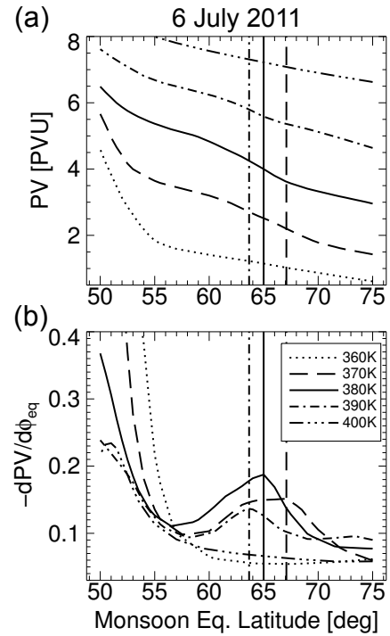
Fig. 18. (a) Potential vorticity with respect to monsoon centered equivalent latitude for 6 July 2011 (calculated from the 5-7 July average), on different levels (360 K, 370 K, 380 K, 390 K, 400 K isentropes). (b) The corresponding PV-gradients with respect to equivalent latitude. Vertical lines show the gradient maxima (transport barriers).
