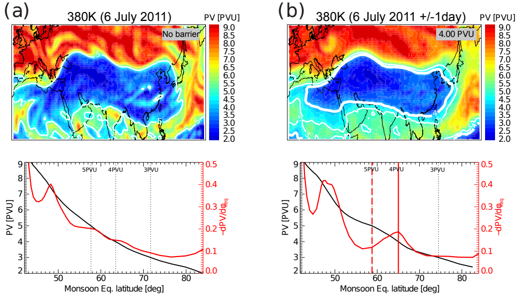
Fig. 15. (a) Potential vorticity map at 380 K on 6 July 2011, in the Asian monsoon region between 10°-60°N and 10°W-160°E (upper panel), and PV as a function of the monsoon centered equivalent latitude (lower panel). Monsoon equivalent latitude \phi_{eq} is calculated from the area within PV contours (see text). Shown is PV(\phi_{eq}) (black) together with the respective PV gradient \partial PV/\partial \phi_{eq} (red). Low PV and large \phi_{eq} indicate the anticyclone center. (b) Same as (a) but for the PV-field averaged between 5 and 7 July 2011. The anticyclone transport barrier, deduced from a local maximum in the PV gradient (see text), is shown as white thick contours (upper panels) and red solid vertical lines (lower panels), respectively. White thin contours (upper panels) and red dashed lines (lower panels) show 5 PVU. Black dashed lines (lower panels) highlight particular PV values. The PV-value of the barrier is given in the grey box.
