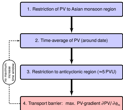
Fig. 19. Method to localize the PV-based transport barrier in the Asian monsoon anticyclone (at 380 K), summarized in four steps.
