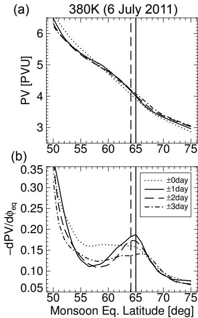
Fig. 16. (a) Potential vorticity with respect to monsoon centered equivalent latitude on the 380 K isentropes, with the PV field averaged over different periods centered around 6 July 2011. (b) The corresponding gradients of PV with respect to equivalent latitude. Vertical lines show the PV-gradient maximum.
