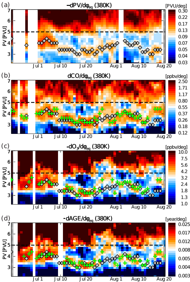
Fig. 112. (a) Time evolution of the gradient of PV with respect to monsoon centered equivalent latitude \phi_{eq} as a function of PV for the period 20 June to 20 August 2011 at 380 K (note the logarithmic color scale). The same is shown for (b) CO, (c) O_3 , and (d) mean age. Symbols show the PV-gradient maximum (grey diamonds), and the CO-gradient maximum (green crosses). The dashed line highlights 5 PVU. Dates without a clear gradient maximum are left white.
