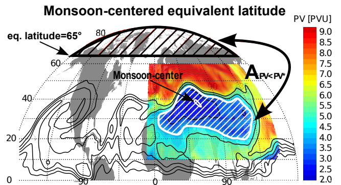
Fig. 14. Illustration of the calculation of monsoon-centered equivalent latitude from the area within PV-contours (see text for details). Color-coded is the PV-field within the Asian monsoon region at 380 K ( 10^\circ\text{N} – 60^\circ\text{N} and 10^\circ\text{W} – 160^\circ\text{E} ) averaged for 5–7 July 2011, with the thick white contour highlighting 4 PVU. The thin white contour encloses the region of lowest PV ( <2.2 PVU) indicating the anticyclone center. The black contours show PV globally.
