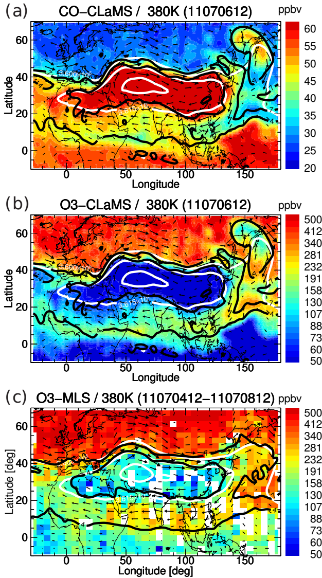
Fig. 12. Maps of (a) CLaMS CO and (b) CLaMS ozone on the 380 K isentropes on 6 July 2011 within the Asian monsoon region. Selected potential vorticity contours are shown in black ( 4, 7 PVU) and Montgomery stream function contours in white ( 3.6 \cdot 10^5, 3.615 \cdot 10^5 \text{ m}^2/\text{s}^2 ). Arrows show horizontal wind. (c) Same but for MLS ozone data sampled during the period 4–8 July 2011, with the MLS data binned into 3^\circ \times 6^\circ latitude/longitude bins (bins without measurements are left white). Meteorological data are taken from ERA-Interim. (Note the logarithmic color scale for ozone.)
