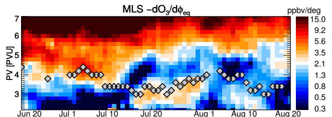
Fig. 114. Time evolution of the gradient of ozone from MLS with respect to monsoon equivalent latitude (based on ERA-Interim PV) for June–August 2011 at 380 K (note the logarithmic color scale). At each date, MLS measurements from 2 days before to 2 days later have been collected, to yield a sufficient coverage of the monsoon region. Grey symbols show the PV-gradient maximum.
