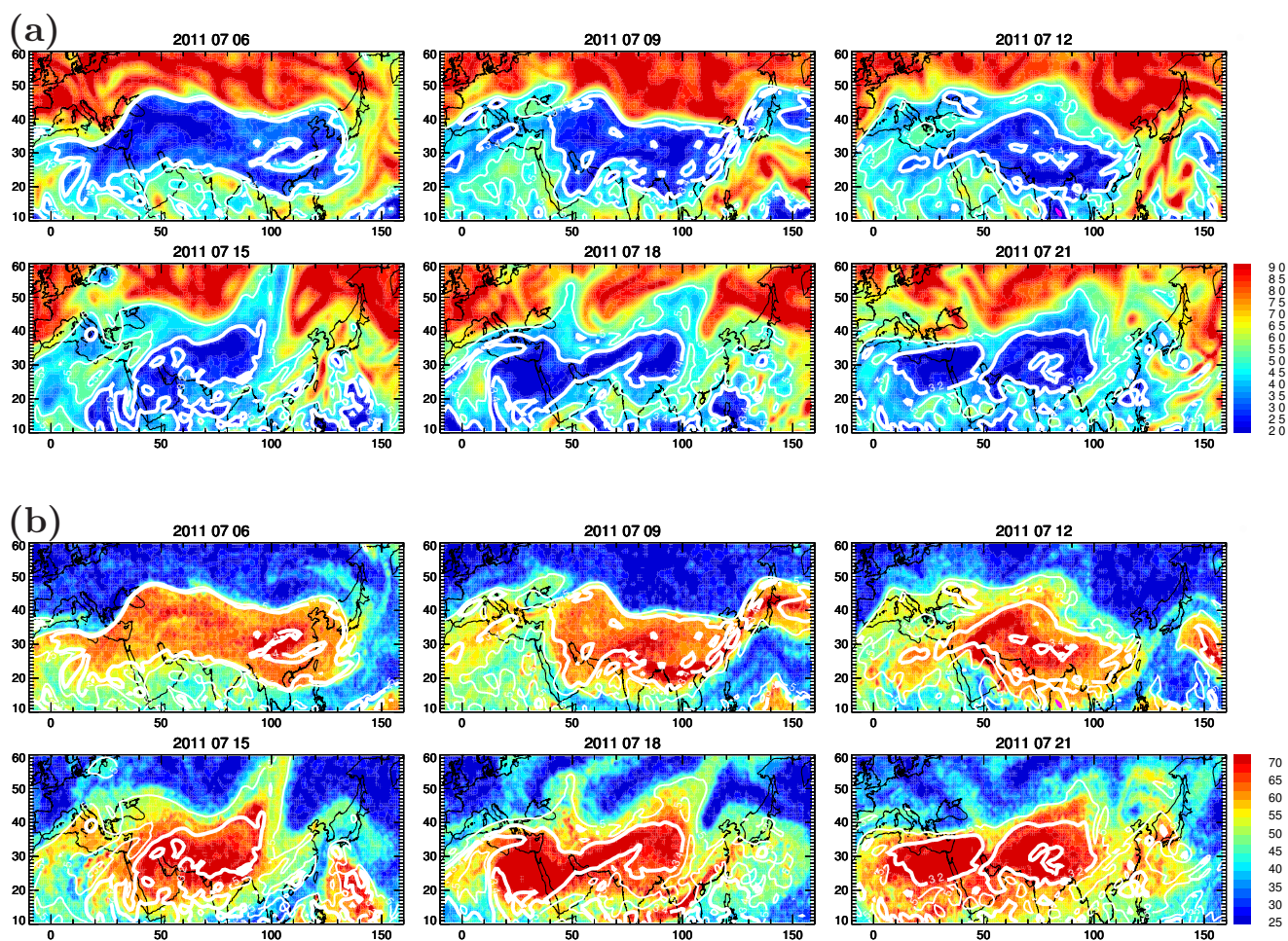
Fig. 110. (a) Potential vorticity maps at 380 K on 6/9/12/15/18/21 July 2011. The thick white contour shows the calculated anticyclone transport barrier (maximum PV gradient), the thin white contour 5 PVU. (b) Maps of CO from CLaMS on the same days, with PV-based transport barrier included as white contours.
