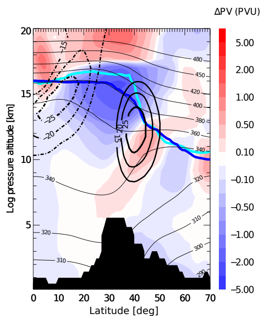
Fig. 11. Meteorological conditions in the Asian monsoon anticyclone (based on ERA-Interim reanalysis). Color shading shows the PV anomaly of the monsoon longitude section (60°–120°E) with respect to the zonal mean, averaged over summer (June–August). Also shown is zonal wind (thick black, solid/dashed positive/negative) and potential temperature (thin black) averaged between 60°–120°E. The first thermal tropopause (calculated using the definition of WMO, 1957) zonally averaged over 0°–360°E is shown as dark-blue, averaged over 60°–120°E as cyan line.
