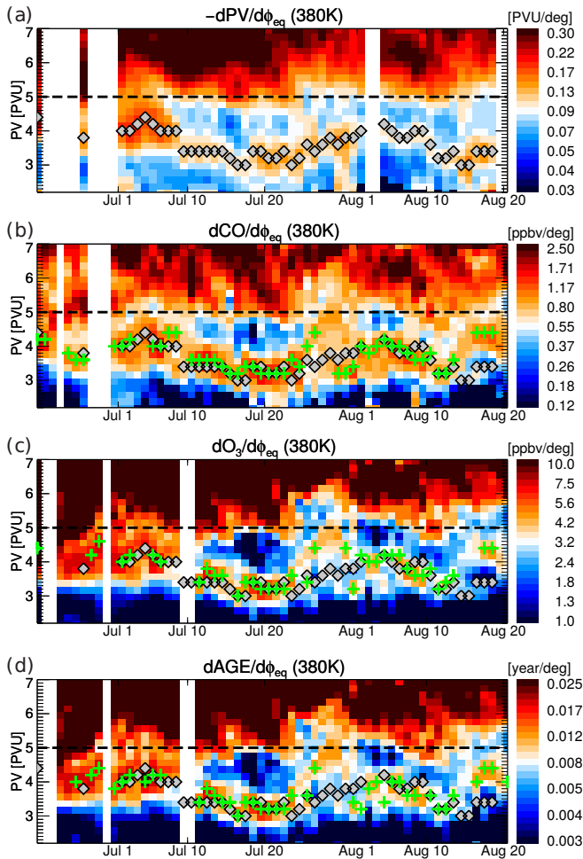
Fig. 12. (a) Time evolution of the gradient of PV with respect to monsoon centered equivalent latitude \phi_{eq} as a function of PV for June–August 2011 at 380 K (note the logarithmic color scale). (b) Same but for CO. Symbols show the PV-gradient maximum (grey diamonds), and the CO-gradient maximum (green crosses). The dashed line highlights 5 PVU. Dates without a clear gradient maximum are left white. (c) Same but for O_3 , and (d) for mean age.
