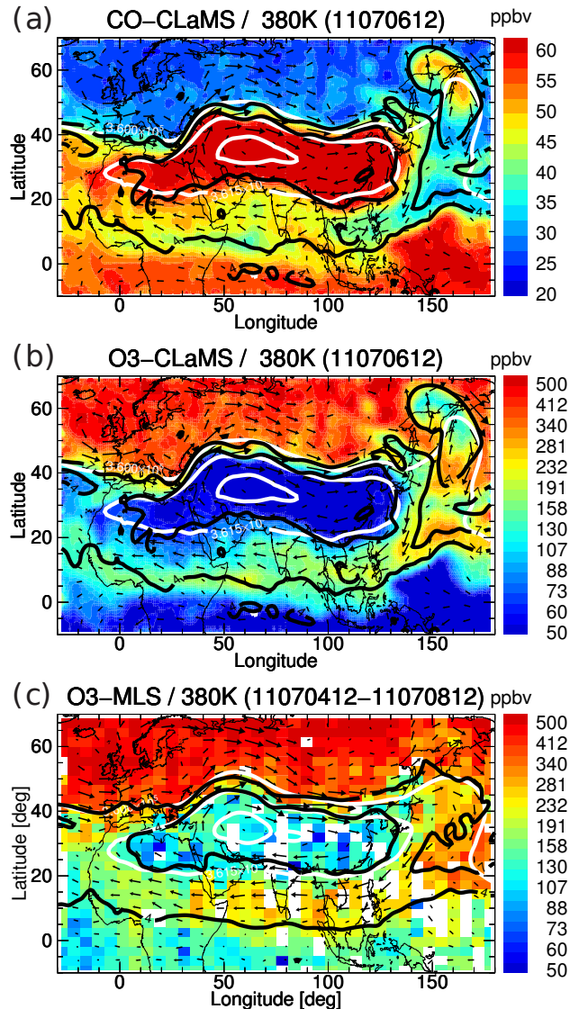
Fig. 2. Maps of (a) CLaMS CO and (b) CLaMS ozone on the 380 K isentrope on 6 July 2011 within the Asian monsoon region. Selected potential vorticity contours are shown in black ( 4, 7\text{ PVU} ) and Montgomery stream function contours in white ( 3.6 \cdot 10^5, 3.615 \cdot 10^5\text{ m}^2/\text{s}^2 ). Arrows show horizontal wind. (c) Same but for MLS ozone during the period 4–8 July 2011, with the MLS data binned into 3^\circ \times 6^\circ latitude/longitude bins (bins without measurements are left white). Meteorological data are taken from ERA-Interim. (Note the logarithmic color scale for ozone.)
