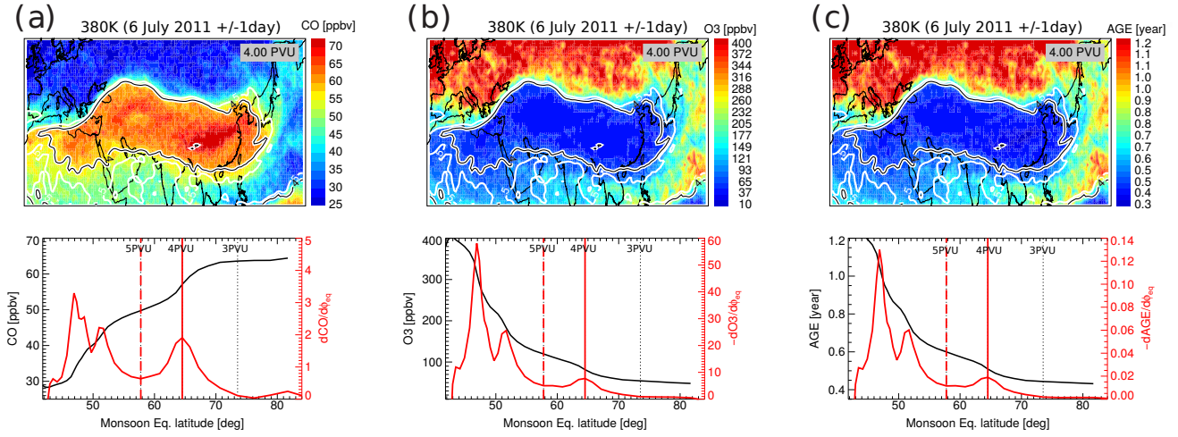
Fig. 11. (a) Map of CO from CLaMS on the 380 K isentrobe, with the thick white contour showing the PV-value of maximum CO-gradient, the black contour showing the PV-value of maximum PV-gradient (thin white line shows 5 PVU), averaged between 5 and 7 July 2011 at 380 K. The bottom panel shows CO from CLaMS versus monsoon centered equivalent latitude (black), and the respective gradient (red). (b) Same for ozone from CLaMS, and (c) for mean age from CLaMS. (The PV values of the maximum gradient are given in the upper panels.)
