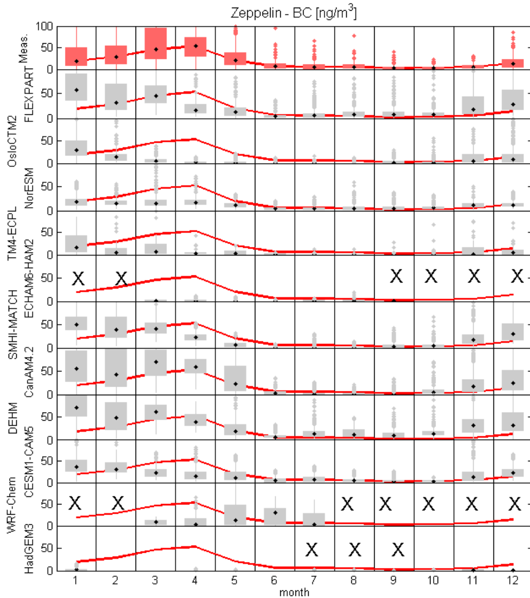
1 2 Figure 4. Observed and simulated mean annual cycle of (equivalent) BC mass concentrations 3 [\text{ng}/\text{m}^3] at the Zeppelin station. Shown is the monthly frequency distributions using data from 4 the years 2008 and 2009. The uppermost panel (red boxes) shows monthly frequency 5 distributions of the observed eBC concentrations. The other panels below (grey boxes) show 6 monthly frequency distributions of the modeled BC concentrations. Black dots depict the 7 monthly median value, the grey boxes span the range between the 25th and 75th percentiles, 8 red and grey dots represent values which are outside the 1.5 fold of this interquartile range (grey 9 lines). The red line connects the monthly medians of the observed eBC concentrations in the 10 uppermost panel and is repeated in all other panels for the convenience of comparing modeled
