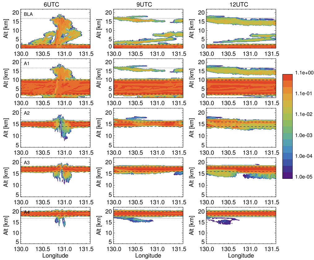
Figure 6. Cross sections of the passive altitude layer tracers at 06:00 UTC (left panels) and 12:00 UTC (right panels). Shown are from top to bottom BLA (initialised below 2 km), A1, A2, A3, and A4. The initialisation layers of the passive tracers are indicated by the dashed lines. The simulated cold point tropopause is shown by the dotted line. Note the changing y-axis scale.
