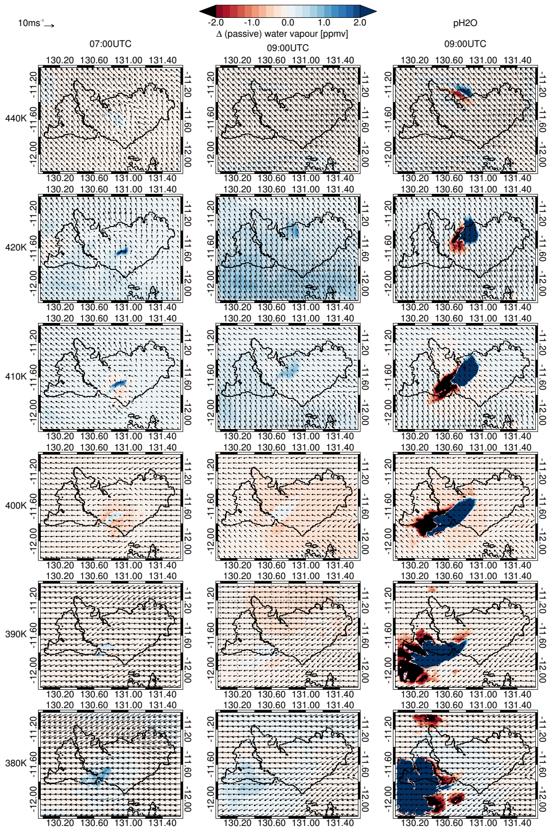
Figure 15. Change in humidity at 07:00 UTC (left column) and 09:00 UTC (middle column) on different potential temperature levels. The right column shows the change of pH 2 O at 09:00 UTC for comparison. Superimposed are the horizontal wind vectors on the respective level.
