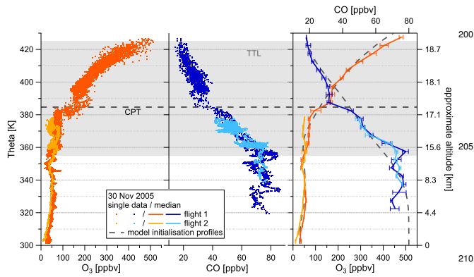
Figure 1. Observed ozone and carbon monoxide mixing ratio profiles (left and middle panel) during the double flight on 30 Nov 2005. On the right, the median observed profiles with the 33 and 67 percentiles (error bars) are shown together with the model initialisation profiles (see Sect. 5). The shading indicates the TTL as defined by Fueglistaler et al. (2009) and the dashed line indicates the cold point tropopause (CPT).
