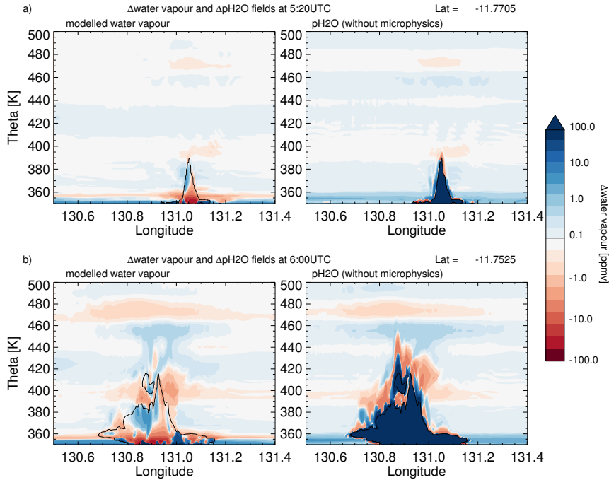
Figure 13. Cross sections of differences in modelled water vapour to the pre-Hector water vapour field (left) and pH2O to the initialisation profile (right) at 05:20 UTC (a) and 06:00 UTC (b).
