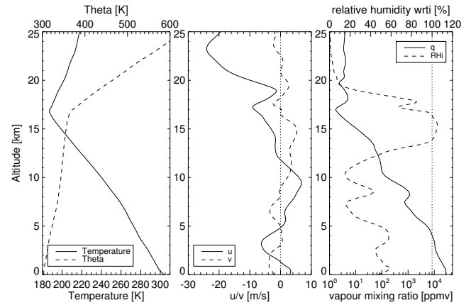
Figure 3. Profile of meteorological parameters prior to Hector development (04:30 UTC). Profiles are averaged over domain 5 and show temperature and potential temperature in the left panel, the u and v wind components in the middle panel, and relative humidity with respect to ice and water vapour mixing ratio in the right panel.
