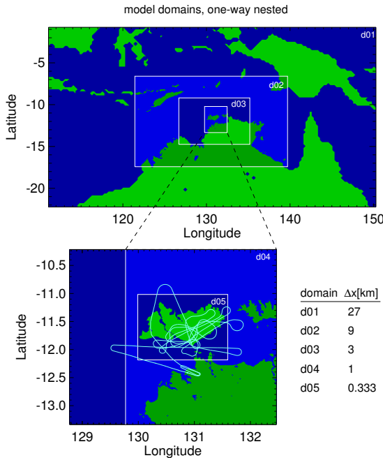
Figure 2. Location of model domains and their horizontal grid spacing. The Geophysica flight path is superimposed in light blue.
