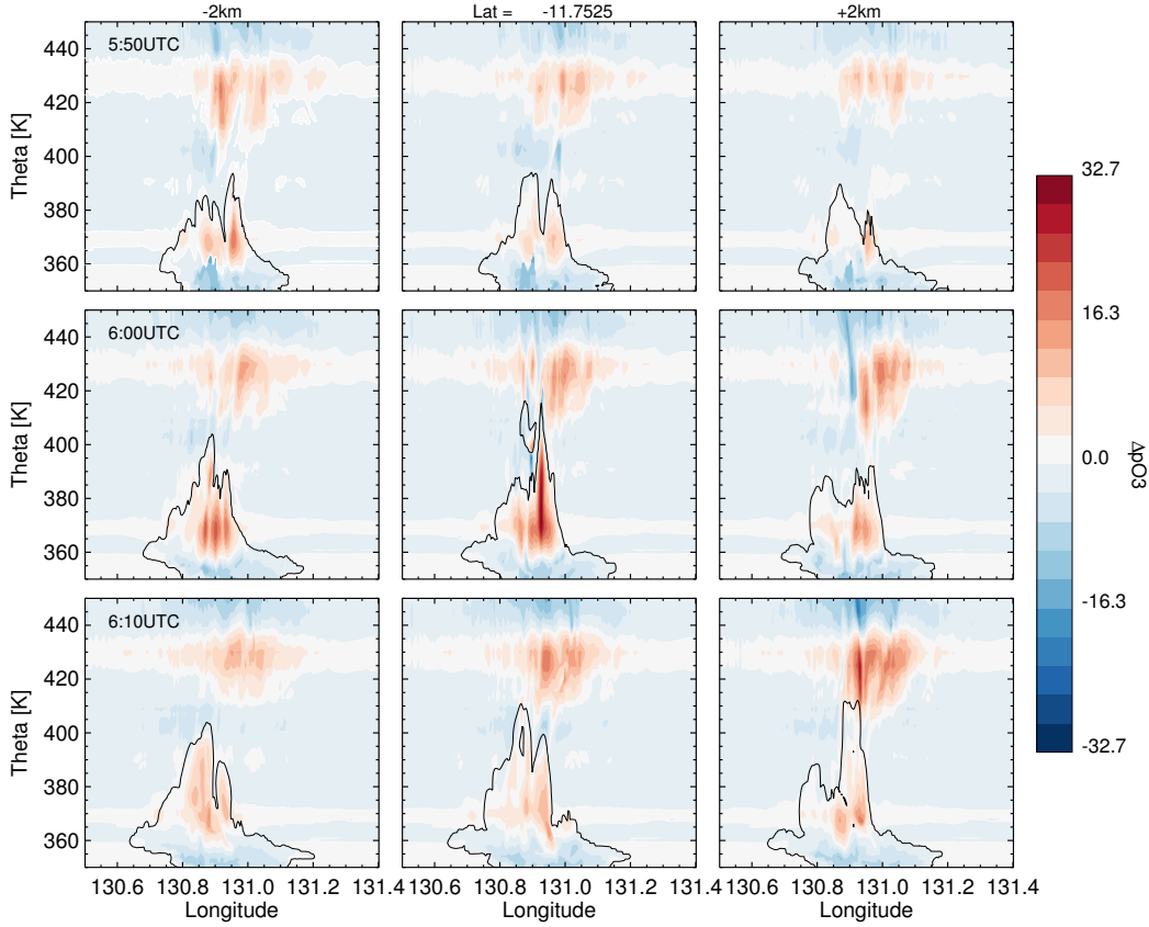
Figure 10. Cross sections of pO3 difference to the initialisation profile ( \Delta pO3 ). By shifting the cross section 2 km to the South/North (right/left) and 10 minutes prior/later (upper/lower panels) the variability of the cloud and the \Delta pO3 field become visible.
