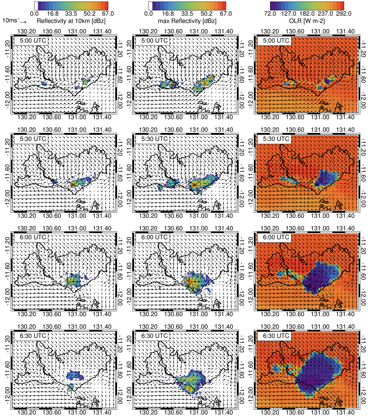
Figure 4. Evolution of 10 m surface winds (arrows), radar reflectivity at 10 km altitude (left panels), column maximum reflectivity (middle panels), and OLR (right panels) as simulated in domain 5.
