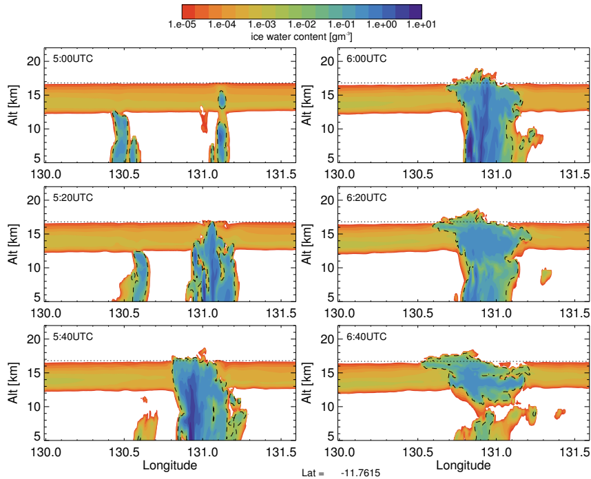
Figure 5. IWC cross sections between 05:00 UTC and 06:40 UTC. The dashed line represents the 0.01 \text{ g kg}^{-1} ice mixing ratio, representing the cloud boundary, and the dotted line indicates the simulated cold point tropopause.
