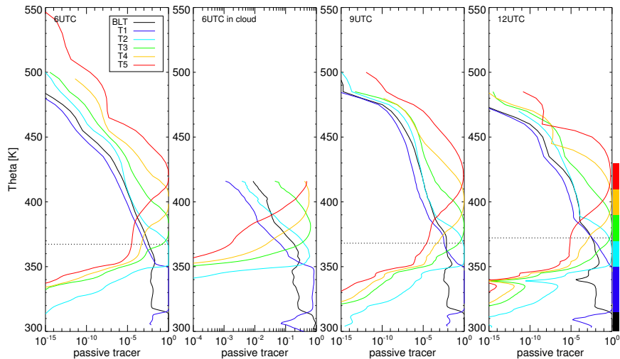
Figure 7. Domain average profiles of the passive tracers BLT, T1 – T5 at 06:00 UTC (left), 09:00 UTC (second from right), 12:00 UTC (right), and in-cloud averages at 06:00 UTC (second from left). The coloured blocks on the right indicate the initialisation layer of the respective passive tracer, in which the tracer have a value of 1, they are 0 outside the layer.
