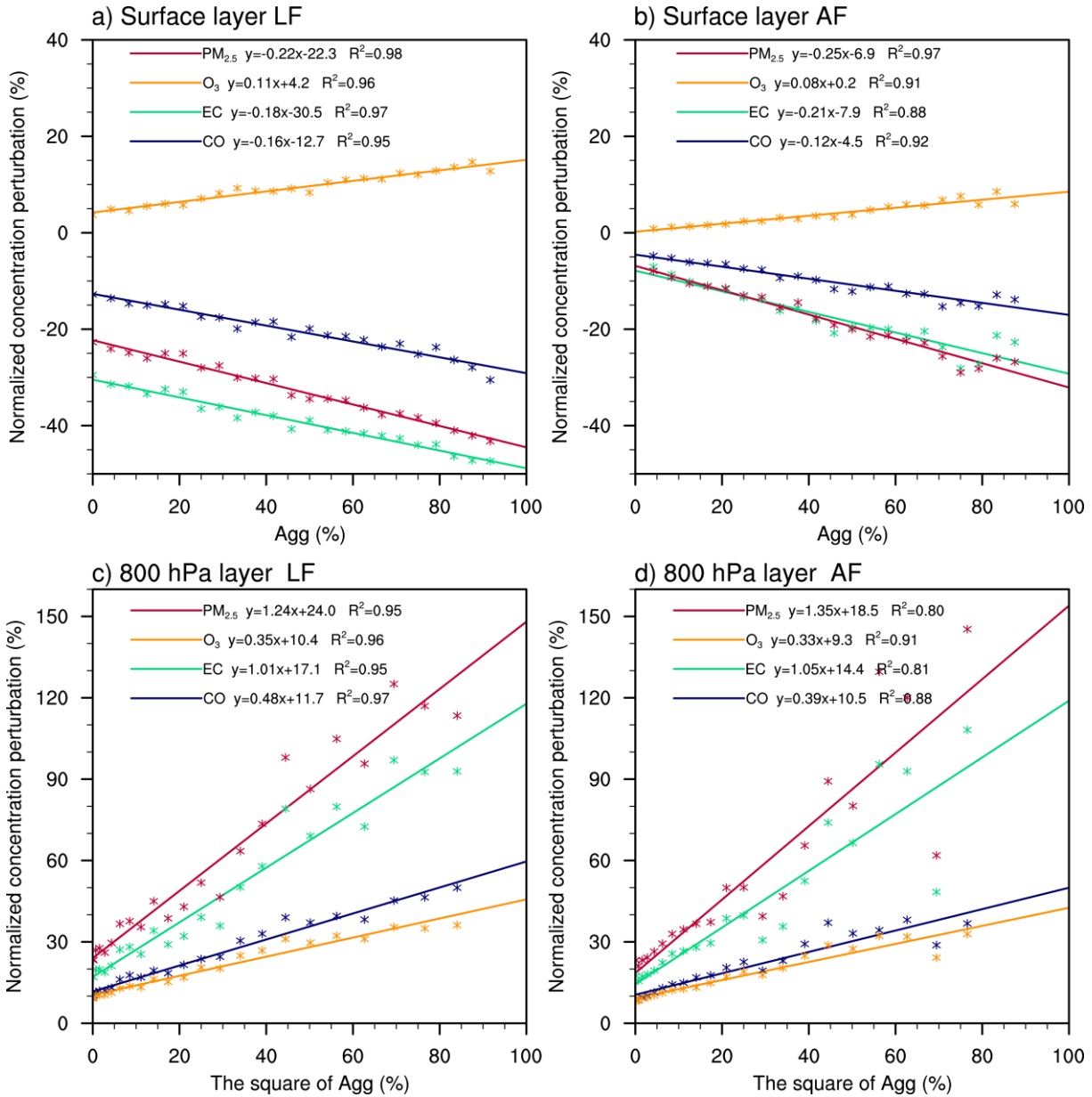
4 Figure 6. Relationship between normalized perturbations of 5-year mean July concentrations 5 of CO, EC, O 3 , and PM 2.5 and Agg at the surface (top), and the square of Agg at 800 hPa 6 (bottom) for the LOCAL forcing (LF, left) and ADJACENT forcing (AF, right). Agg is 7 defined as the occupation rate of the newly urbanized cells to the surrounding 24 (5 × 5 - 1) 8 cells. Linear regression results are also shown.
