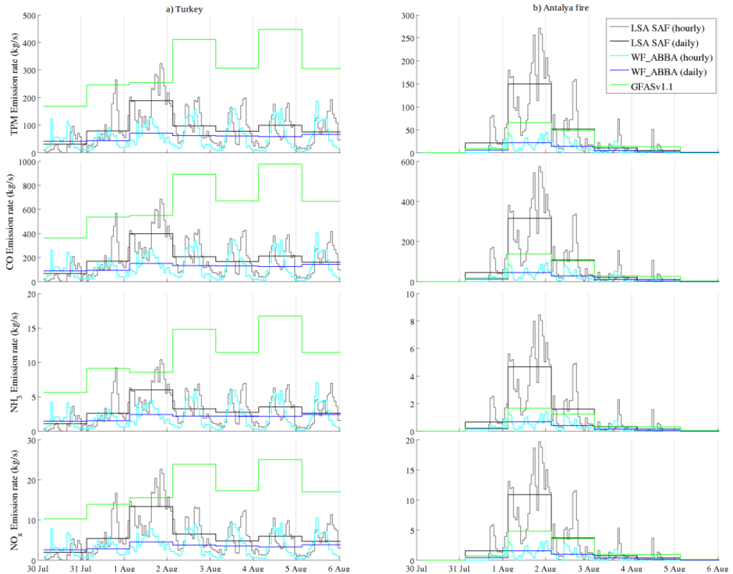
Figure 3. TPM, CO, NH 3 , NO x emission rate rates observed over Eastern the eastern Mediterranean (a) and over the Antalya fire (b) from 30 July to 6 August 2008. Cyan and blue line: lines are the hourly and daily WF_ABBA FRP derived. Grey and black line: lines are the hourly and daily LSA SAF FRP derived. Green line is the GFASv1.1.
