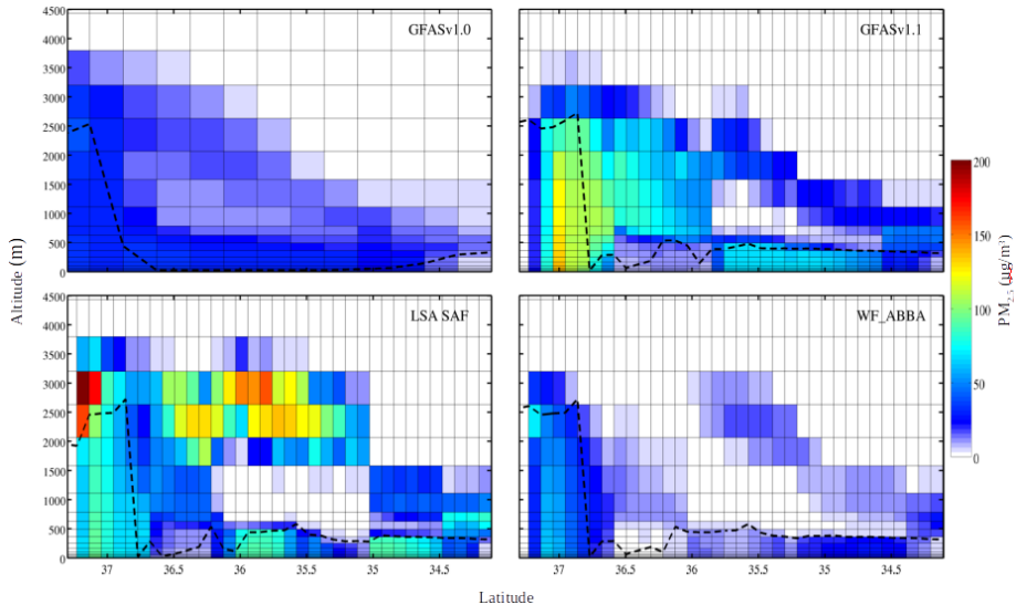
Figure 7. 1 August 2008, 15:00 LT. Vertical cross section, across the concurrent maximum simulated AOT, showing the changes in the PM 2.5 concentration across the main plume of Antalya fire for the CMAQ simulations performed with GFAS1.0 (a), GFAS1.1 (b), LSA SAF (c) and WF_ABBA (d) based fire emission inventories. The changes in the PM 2.5 concentration are calculated by subtracting concentrations from simulations without fires. Black The black dashed line defines the PBL.
