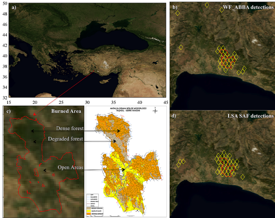
Figure 1. (a) Study area. (c) Burned area as reported by the Antalya Forestry department (right) and over a MODIS Blue Marble image (left). (b) WF_ABBA (MSG-SEVIRI) detections of the Antalya fire. (d) LSA SAF (MSG-SEVIRI) detections of the Antalya fire.
