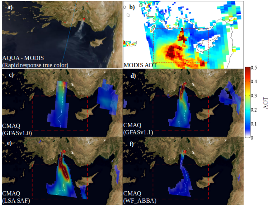
Figure 6. (a) MODIS (true color composite from visible wavelengths) over the Eastern - eastern Mediterranean basin on 1 August 2008 at 14:30 LT . (b) Concurrent MODIS level 2 aerosol optical thickness product . Concurrent CMAQ simulated changes in AOT due to fires made by using GFAS1.0 (c), GFAS1.1 (d), LSA SAF (e) and WF_ABBA (f) based fire emission inventories. The changes in the AOT are calculated by subtracting concentrations from simulations without fires. The white dashed line connects the cells of the model grid having the maximum simulated AOT along the Antalya fire plume. MODIS AOT colorscale is the same as the one for the simulated changes in AOT in the different simulations .
