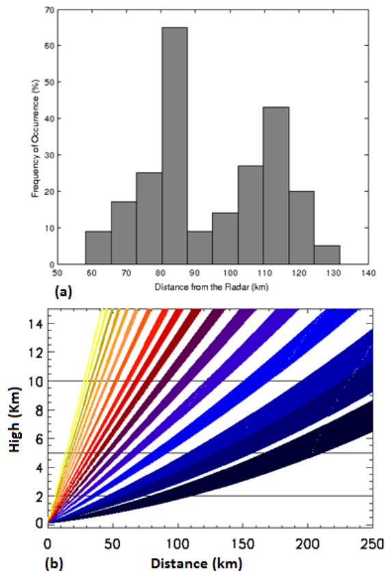
Fig. 1. (a) Frequency histogram of distance from the radar of elevations greater than 126 meters; (b) Cross section of the volumetric scan strategy for the S-band Radar in Manaus. Each colored band represents
