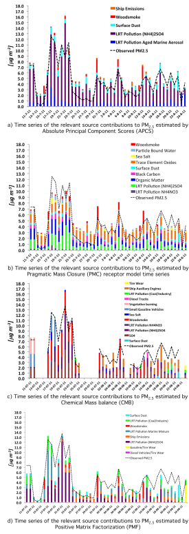
Fig. 3. Four receptor model source apportionment panel
