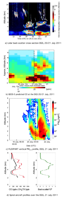
Fig. 5. Lidar_GEOS 5_FLEXPART_Aircraft Spiral panel
