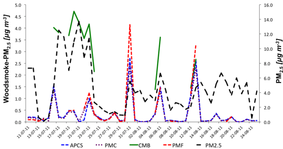
Fig. 4. Four model woodsmoke time series plot
