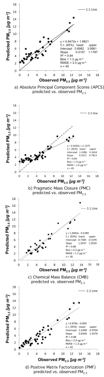
Fig. 1. Four receptor model comparison predicted vs. observed panel
