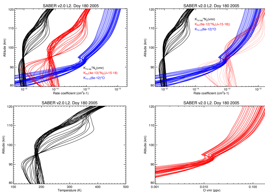
Fig. 1. Calculation of VT(CO 2 -N 2 ), new proposed mechanism (RV CO 2 -N 2 ), and VT (CO 2 -O) deactivation rates for one solstice day. Temperatures and O vmr are also plotted.
