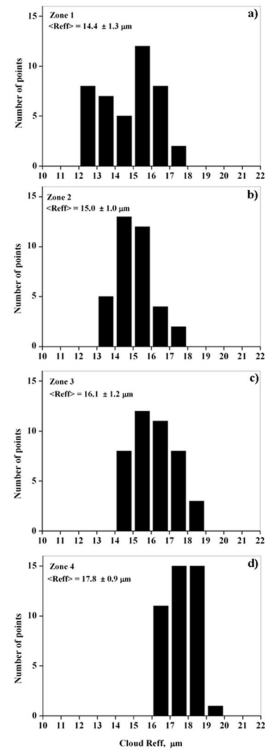
Fig. 1. The histograms of effective particle radius (Reff) for liquid water clouds in the specified zones 1 – 4 along SAL, based on MODIS Level 3 gridded monthly data with resolution 1x1 degr. in July 2010.
