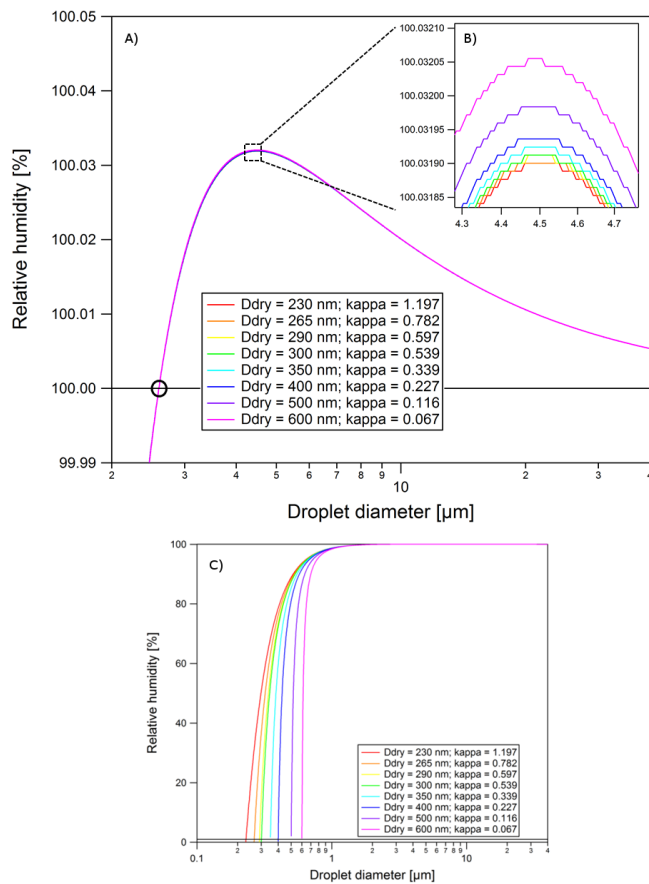
Fig. 1. Köhler curves for different pairs of dry diameter and \kappa value, chosen in such a manner that all curves cross \text{RH}=100\% at a droplet diameter of 2.6 \mu\text{m} . This intersect is
