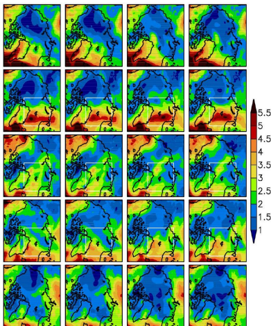
New Fig. 13. Pan-Arctic distribution of synoptic-scale variability on time scales from 1–3 days expressed as filtered temporal standard deviation of 6 hourly mean sea level pressure (hPa) for November 2007 (upper row) until March 2008 (lower row) and December, January and February in between. From left to right ECMWF operational analyses, HIRHAMf12 simulations, HIRHAM clima simulations with b = 5 , and HIRHAM b10 with b = 10 .
