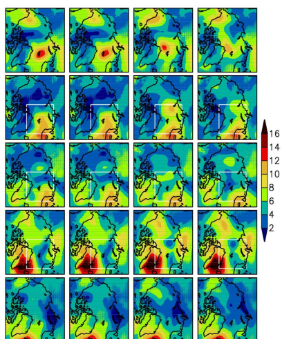
New Fig. 15. Pan-Arctic distribution of baroclinic-scale variability on time scales from 10–20 days expressed as filtered temporal standard deviation of 6 hourly mean sea level pressure (hPa) for November 2007 (upper row) until March 2008 (lower row) and December, January and February in between. From left to right ECMWF operational analyses, HIRHAM f12 simulations, HIRHAM clima simulations with b = 5 , and HIRHAM b10 with b = 10 .
