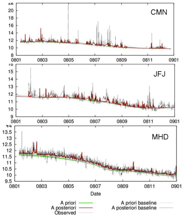
Fig. 4. Comparison between the observed (grey) and modelled (red) time series at the three stations.
