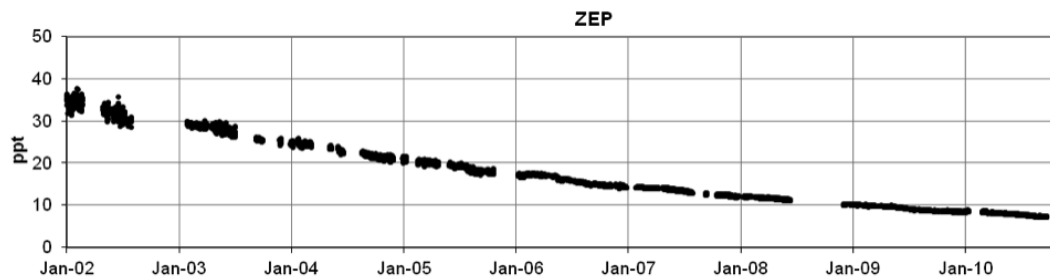
Fig. 2. Methylchloroform time series at Zepellin station (ZEP)
