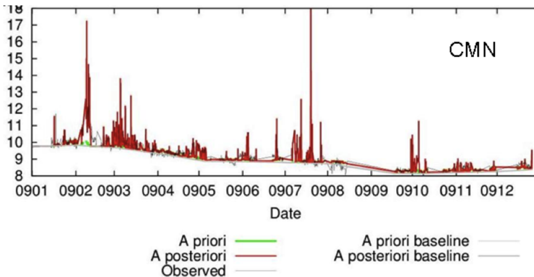
Fig. 5. Comparison between the observed (grey) and modelled (red) time series at CMN obtained using the PSA
