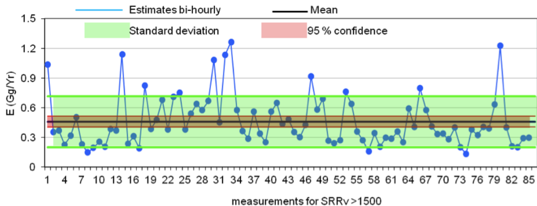
Fig. 3. Time series of estimated emissions for JFJ for a SRRv threshold >1500
