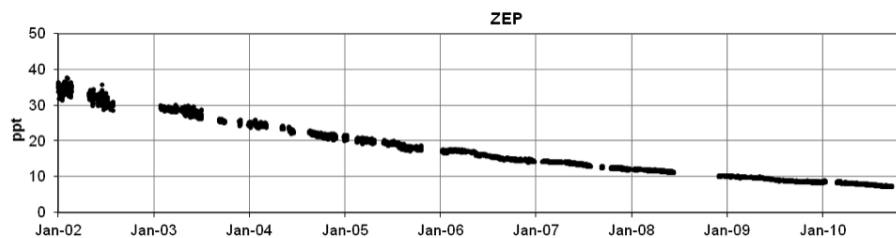
Fig. 2. Methylchloroform time series at Zepellin station (ZEP)
