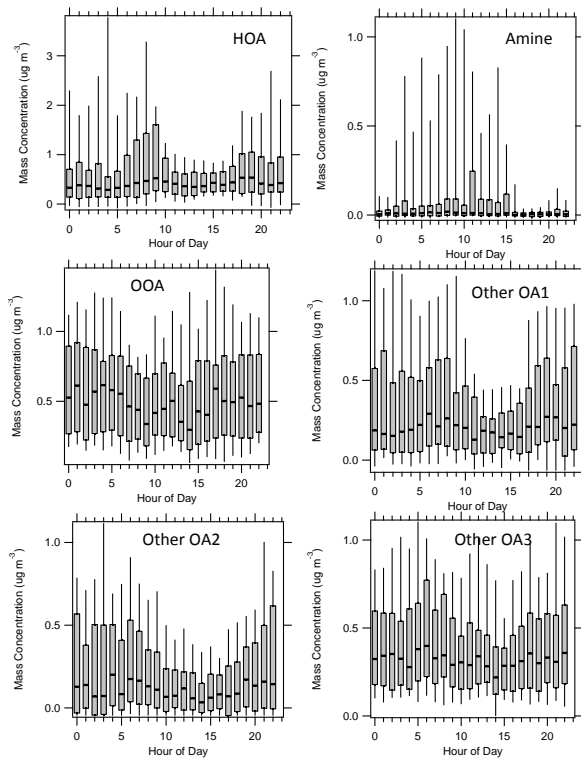
Fig. 5. Figure S-3.11 added to the Supplement. Diurnal trends for the PMFOrG MS six factor solution.
