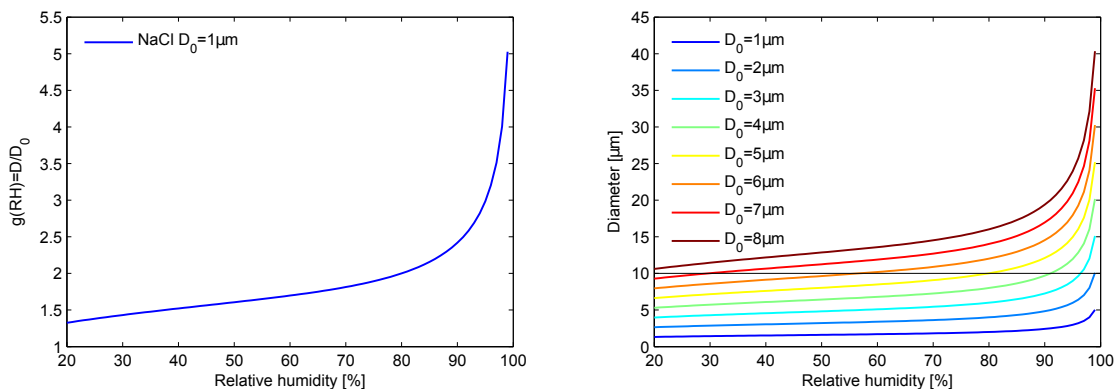
Fig. 1. Left: The hygroscopic growth factor for pure NaCl vs. RH ( D_p of 1 \mu\text{m} ). Right: The resulting diameter change for different dry diameters. The black line indicates as an example the PM10 size cut.
