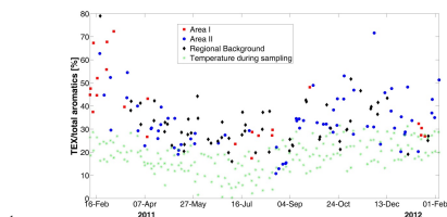
Figure 8. Temporal variation of the concentration ratios of the sum of toluene, ethylbenzene and xylenes (TEX) to total aromatics from air masses arriving at Welgegund after passing
