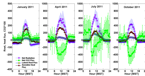
1 Figure 2: Average diel net radiation (downwelling minus upwelling), latent heat flux, sensible 2 heat flux and net CO 2 flux for four representative months. All properties were measured from 28 3 m at the top of the chemistry tower in 2011. Each data point represents a 30 minute average for 4 that time period. The y-axis limits are the same for each plot except for January, where the scale 5 is 1/2 of the other three months. The shaded area for net radiation and error bars for CO 2 flux 6 represent \pm 1 standard deviation. Error bars for sensible and latent heat fluxes have been omitted 7 for clarity. 8
