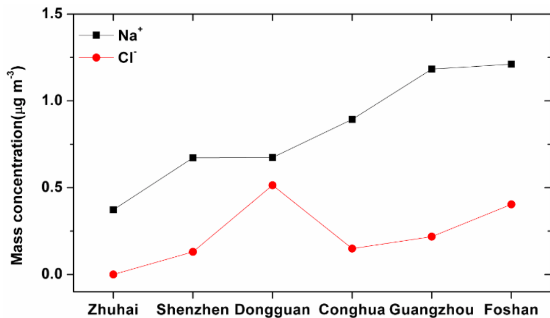
Fig. 7. The mass concentration of \text{Na}^+ and \text{Cl}^- in \text{PM}_{2.5} samples collected in the 6 sites
