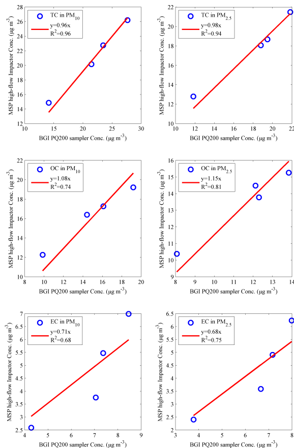
Fig. 1. Comparison between the measurement results of MSP high-flow Impactor and BGI PQ200 sampler
