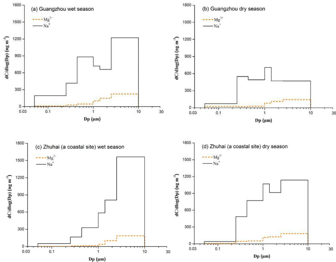
Fig. 5. size distributions of \text{Na}^+ and \text{Mg}^{2+} at Guangzhou during (a) wet season and (b) dry season in this study as well as that at a coastal site (Zhuhai) at PRD region during (c) wet season and (d) dry season
