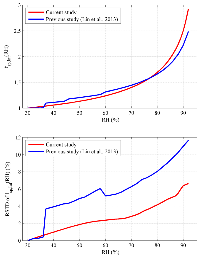
Fig. 8. Comparison between the estimated f_{sp}(RH) based on the method proposed in the current study and the one in a previous study
