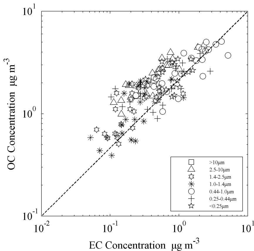
Fig. 4. Comparison between the mass of OC and EC
