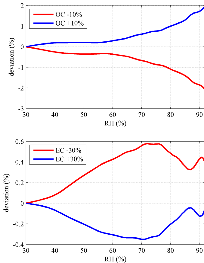
Fig. 2. Deviation of f_{sp}(RH) due to the mass variations of OC and EC
