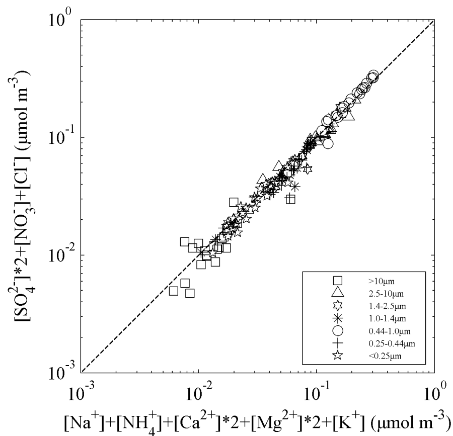
Fig. 3. The balance of charge equivalence between the cations and anions
