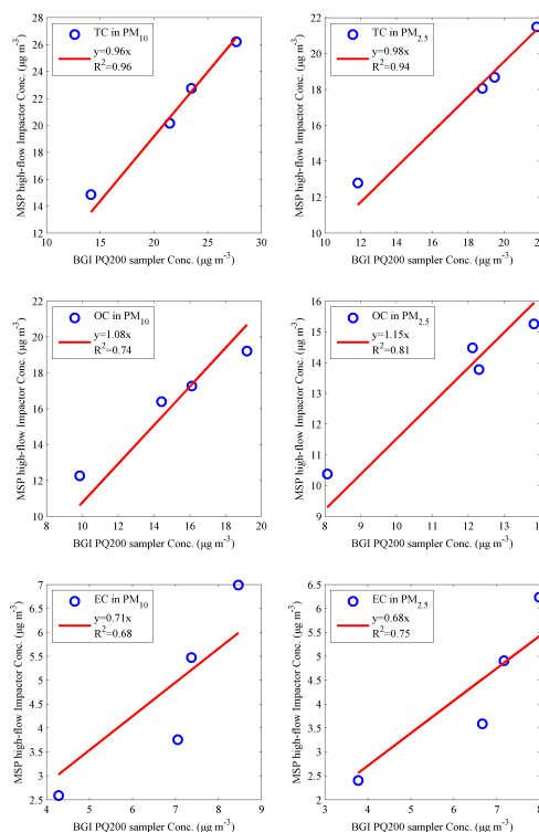
Fig. 1. Comparison between the measurement results of MSP high-flow Impactor and BGI PQ200 sampler
