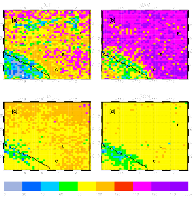
Fig. 2. MOPITT CO total column in vmr
