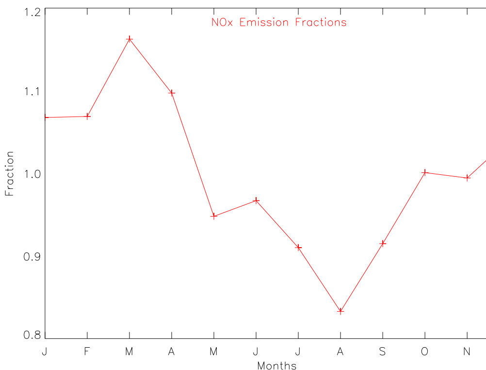
Fig. 1. NO x emissions seasonal cycle, based on Visschedijk et al., (2007), which is applied to AQUUM's NO x emission annual totals.
