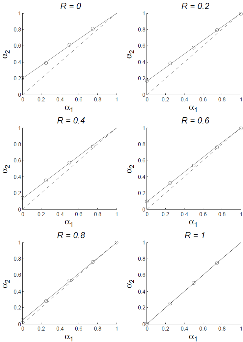
2 Fig. 1. The dependence of \alpha_2 on \alpha_1 for cloud fractions (in adjacent grid boxes) that are 3 uniformly distributed, where the vertical correlation coefficient in cloud cover \rho = 1 and the 4 horizontal correlation coefficient in cloud cover is R (solid line). The dashed line is where 5 there would be no scale dependence to \alpha (i.e. \alpha_2 = \alpha_1 ). The circles are values given by 6 simulation.
