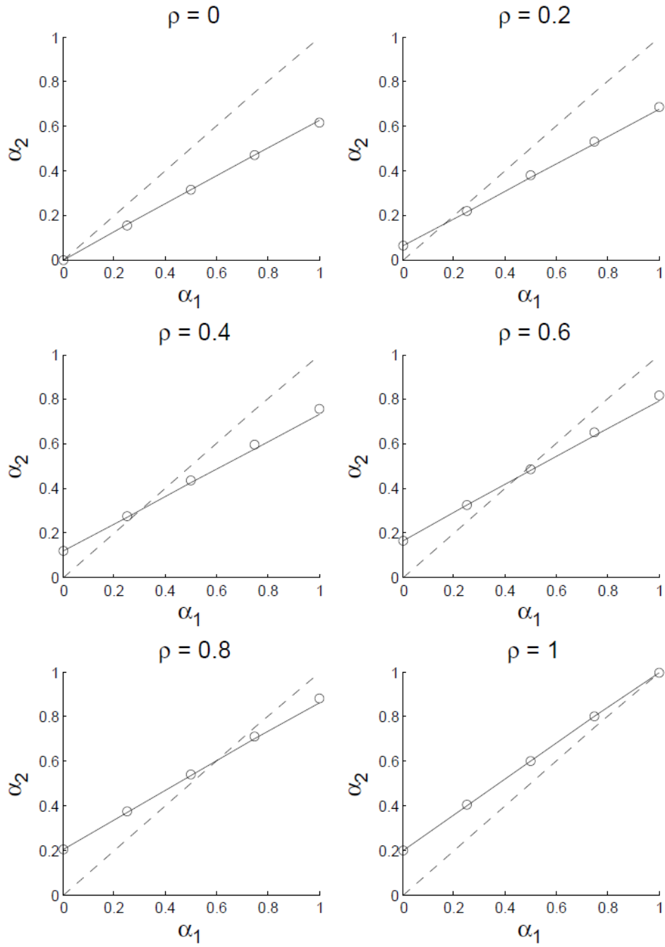
3 Fig. 2. The dependence of \alpha_2 on \alpha_1 for cloud fractions that are uniformly distributed (solid 4 line), where the horizontal correlation coefficient in cloud cover is R = 0 , and the vertical 5 correlation coefficient in cloud cover is \rho . The dashed line is where there would be no scale 6 dependence to \alpha (i.e. \alpha_2 = \alpha_1 ). The circles are values from simulation.
