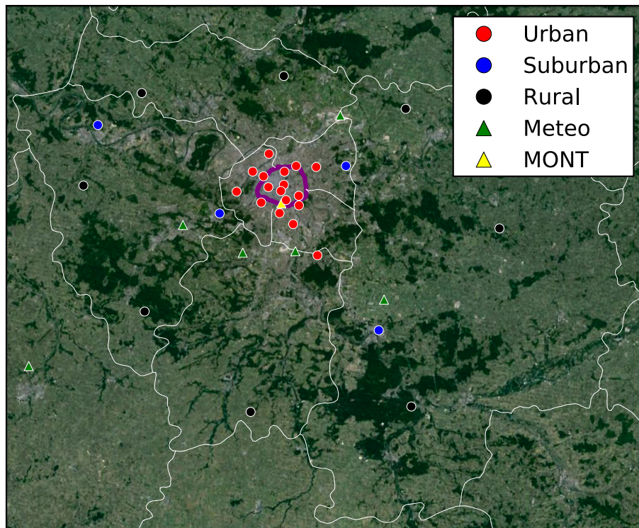
Fig. 1. Local scale (IdF) simulation domain, with the city of Paris in the center (area enclosed in the purple line). Circles correspond to sites of the local air-quality monitoring network (AIR-PARIF) with red for urban, blue for suburban and black for rural. Triangles correspond to the meteorological stations (the yellow triangle correspond to the Montsouris meteorological located in the city center).
