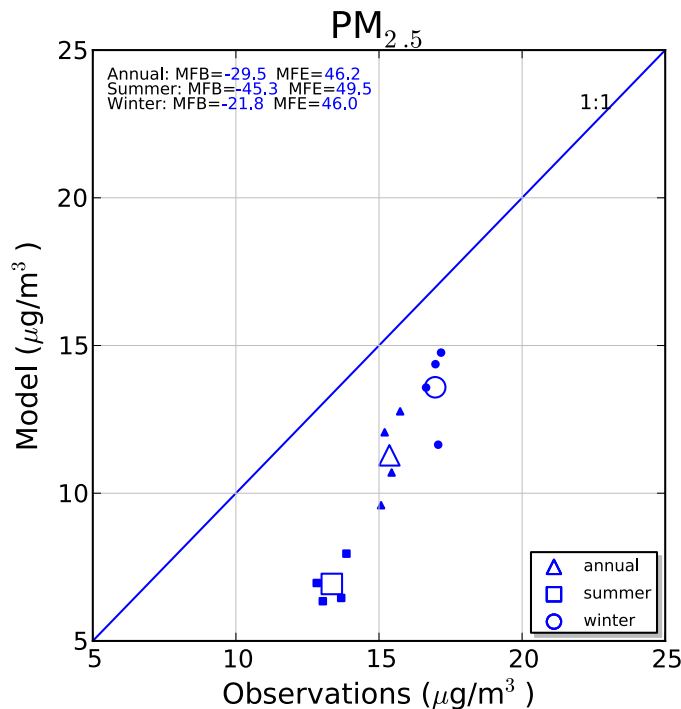
Fig. 3. Scatter plot of mean daily PM 2.5 from the model run during summer (JJA), winter (DJF) and on annual basis against observations. Full small markers represent concentrations at individual stations while large hollow markers stand for the aggregated value.
