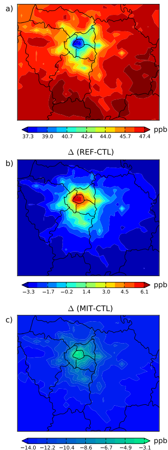
Fig. 4. Present time ozone daily maximum (ppb) of 8 h running means averaged over the April–August period (a) and differences between the CTL run and the REF (b) and MIT projections (c) .
