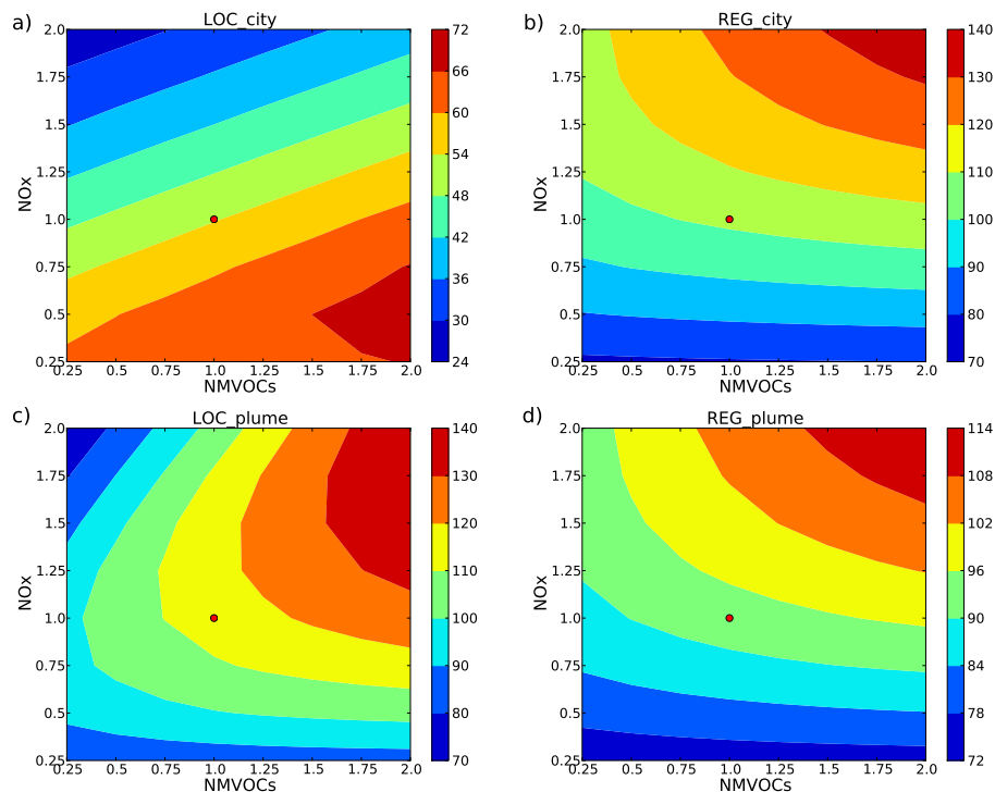
Fig. 5. Isocontours of maximum ozone concentrations over downtown Paris (top panels) and over the entire modelling domain (IdF) (bottom panels) as a function of ozone precursor emissions. Axis units are the coefficients of emission changes with respect to their baseline values (point 1.0, 1.0) are given on both axes. Isopleths on the left are modelled with the LOC simulation and on the right with the REG simulation.
