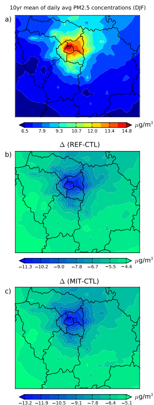
Fig. 7. Wintertime (DJF) PM 2.5 daily average fields ( \mu\text{g}\text{m}^{-3} ) for the control simulation (a) and the differences between the latter and the REF (b) and MIT (c) future projections.
