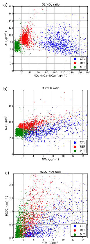
Fig. 6. Ozone chemical regime indicators for the control run and the two future projections. Dots represent daily means averaged during the ozone period over the grid-cells of the downtown Paris area.
