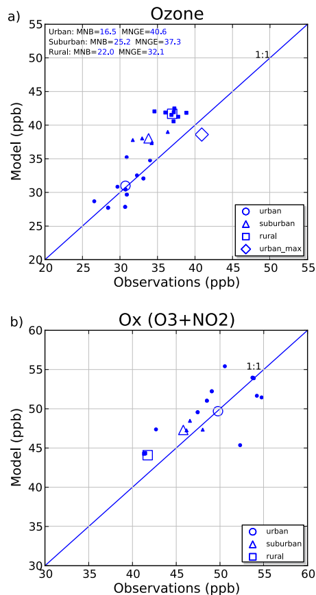
Fig. 2. Scatter plots of mean daytime ozone (a) and O x (b) during the April to August period from the model run against observations. Full small markers represent concentrations at individual stations while large hollow markers stand for the aggregated value. “Urban_max” stands for the daily maximum of an 8 h running average.
