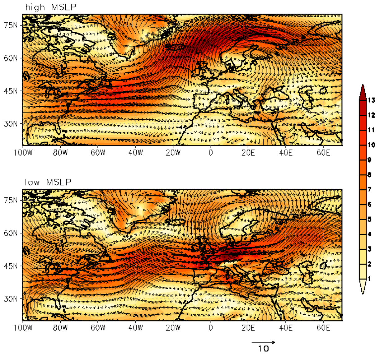
696 697 Fig. S3: Same as in Fig. S1, but for high and low MSLP conditions. 698 699
