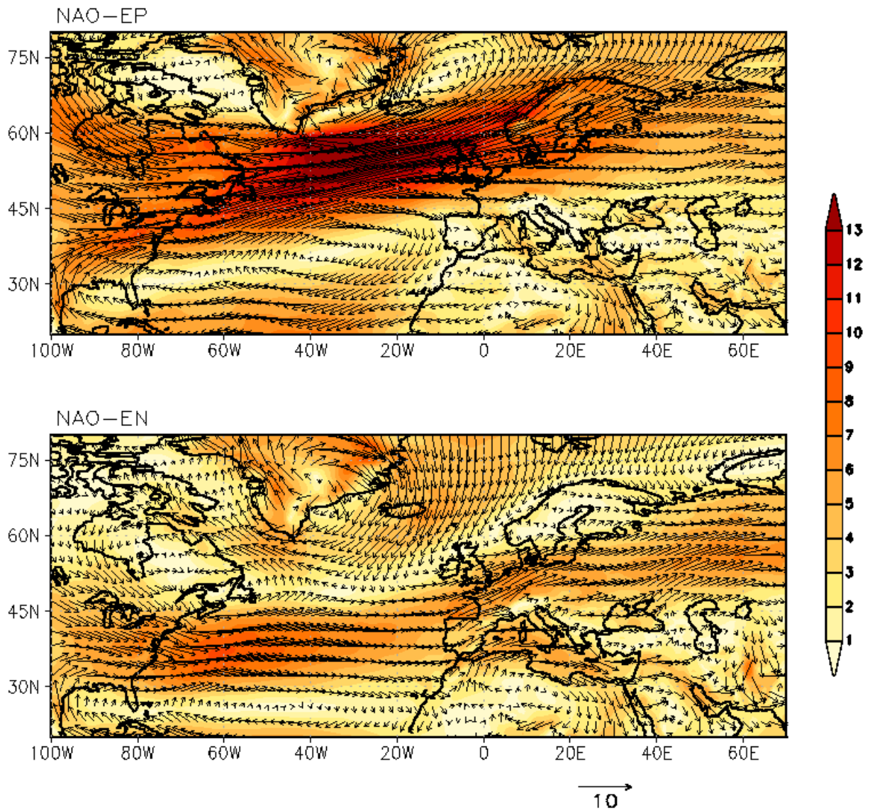
712 713 Fig. S4: Same as in Fig. S1, but for the enhanced positive and negative phases of NAO. 714 715 716 717 718 719 720 721 722 723
