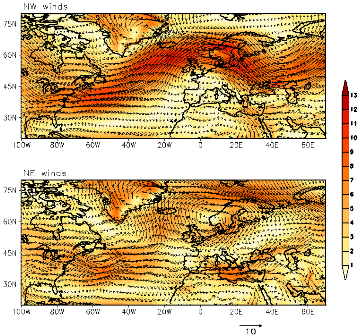
662 663 Fig. S1: Broader view of atmospheric circulation patterns at 850 hPa when winds are NW and NE over 664 the center of the study area (45-80N, 10W-40E). 665
