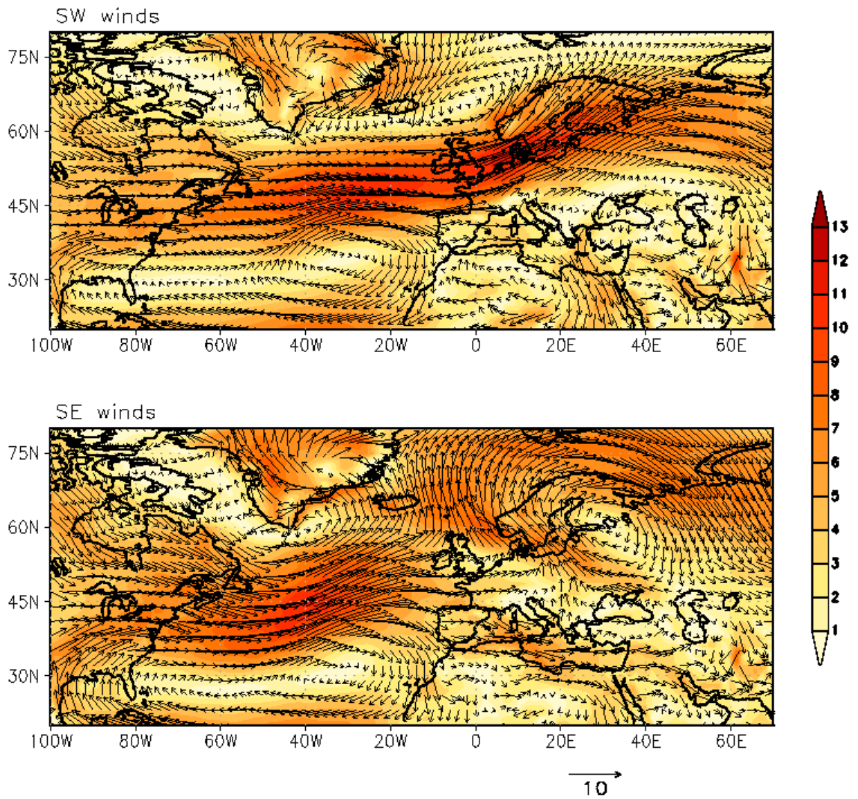
Fig. S2: Same as in Fig. S1, but for SW and SE winds.
