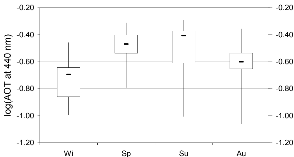
Fig. 1.2: seasonal variations of the AOT at 440 nm. Dashes indicate median values, rectangles median \pm 1 standard deviation, and whiskers the 5th and 95th percentiles.
