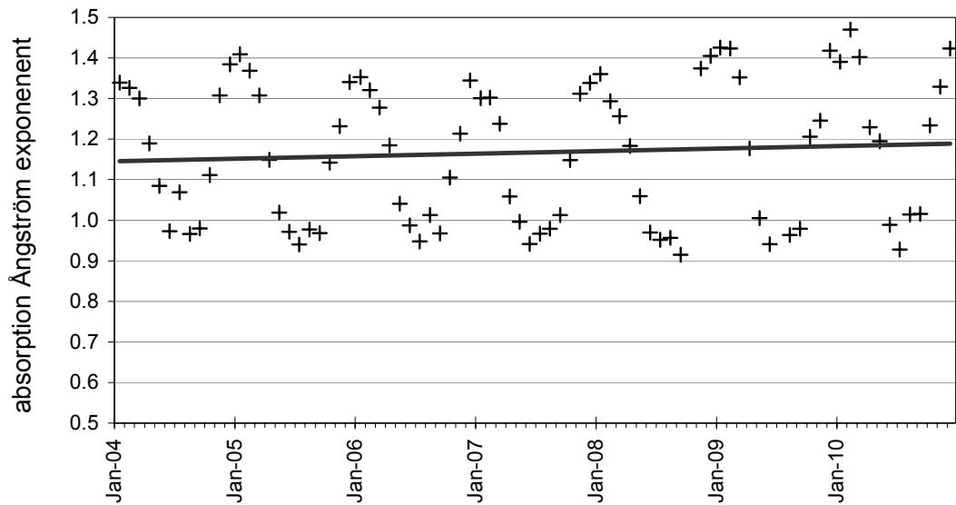
Fig. 2.1: variations in the absorption Ångström exponent at IPR, calculated from the Aethalometer absorption raw data at 7 wavelengths from 370 to 950 nm.
