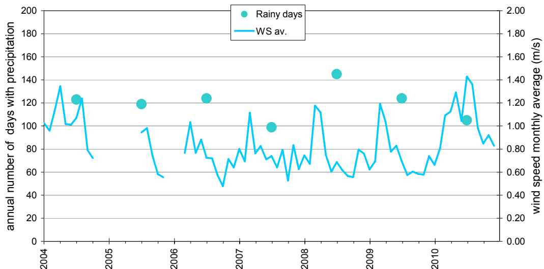
Fig. 1.1.: variations in relevant meteorological variables during the studied period.
