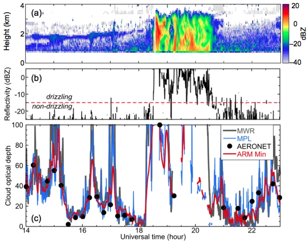
Figure 5. Same as Fig. 4, but for 2 May 2007. Heavy precipitation occurs at 18.5–20.5 UTC.
