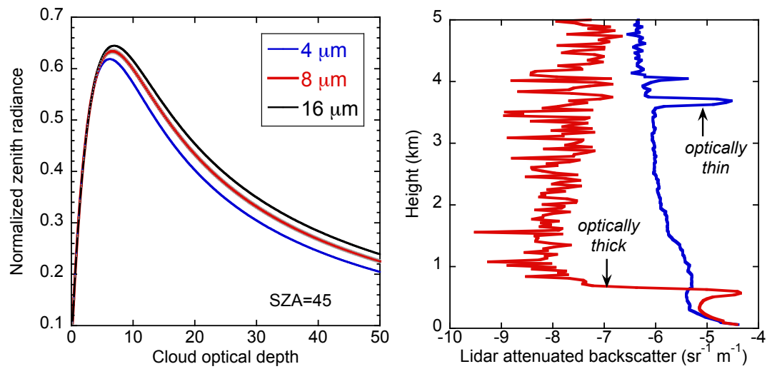
Figure 1. (a) Plot of calibrated solar background light in lidar measurements versus cloud optical depth at 523-nm wavelength and solar zenith angle (SZA) of 45° for cloud effective radius of 4, 8 and 16 μm. (b) Vertical profiles of logarithm (with base 10) lidar attenuated backscatter signals measured on 15th June 2007 at the ARM Oklahoma site at 19 UTC for optically thick clouds, and at 23.5 UTC for optically thin clouds.
