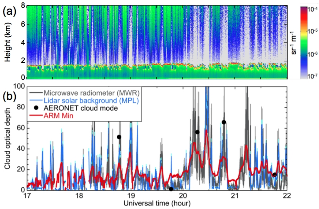
Figure 3. (a) Attenuated backscatter signals from micropulse lidar on 19 April 2005. (b) Time series of cloud optical depth retrieved from microwave radiometer (MWR), lidar solar background signals from micropulse lidar (MPL), AERONET cloud-mode observations, and ARM Archive Min retrievals (using narrowband irradiance measurements). MWR-based retrievals (grey lines) are based on an assumed cloud effective radius of 8 \mu\text{m} ; gray error bars denote lower and upper limits for MWR values, respectively corresponding to a change in droplet effective radius from 6 to 14 \mu\text{m} .
