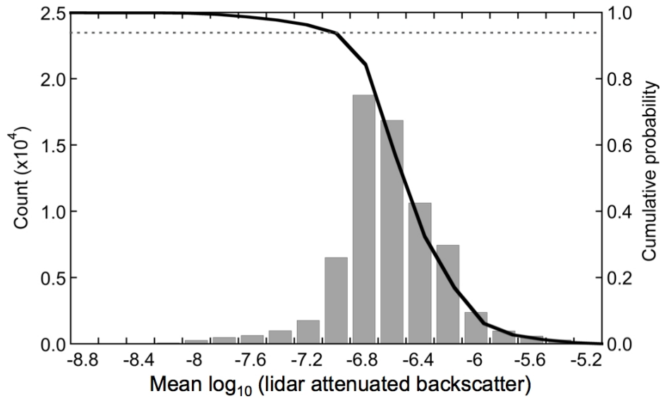
Figure 2. Histogram of \beta_{\text{ct},1\text{km}} (the mean logarithm (with base 10) lidar backscatter from the cloud top to 1 km above) and the corresponding cumulative probability (solid line) accounted from the larger end of \beta_{\text{ct},1\text{km}} for clear sky at the ARM Oklahoma site in 2005. The dashed line represents the 94% cumulative probability.
