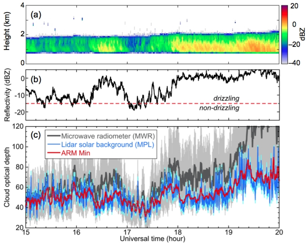
Figure 4. (a) Time series of radar reflectivity profiles on 10 April 2007. (b) Cloud-base reflectivity indicating the presence of drizzle. (c) Time series of cloud optical depth retrieved from microwave radiometer (MWR), lidar solar background signals from micropulse lidar (MPL) and ARM Archive Min retrievals. Grey error bars denote lower and upper limits for MWR values, respectively corresponding to a change in droplet effective radius from 6 to 14 \mu\text{m} . Note that AERONET cloud-mode observations were unavailable for this day
