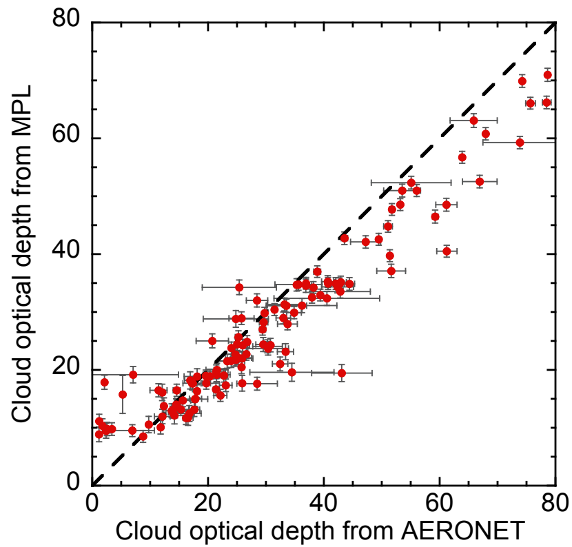
Figure 7. Scatterplot for intercomparison of cloud optical depths retrieved from solar background signals received by micropulse lidar (MPL) and those from the AERONET cloud-mode product. The error bars represent one standard deviation of retrievals, while the black dashed line represents the 1:1 line.
