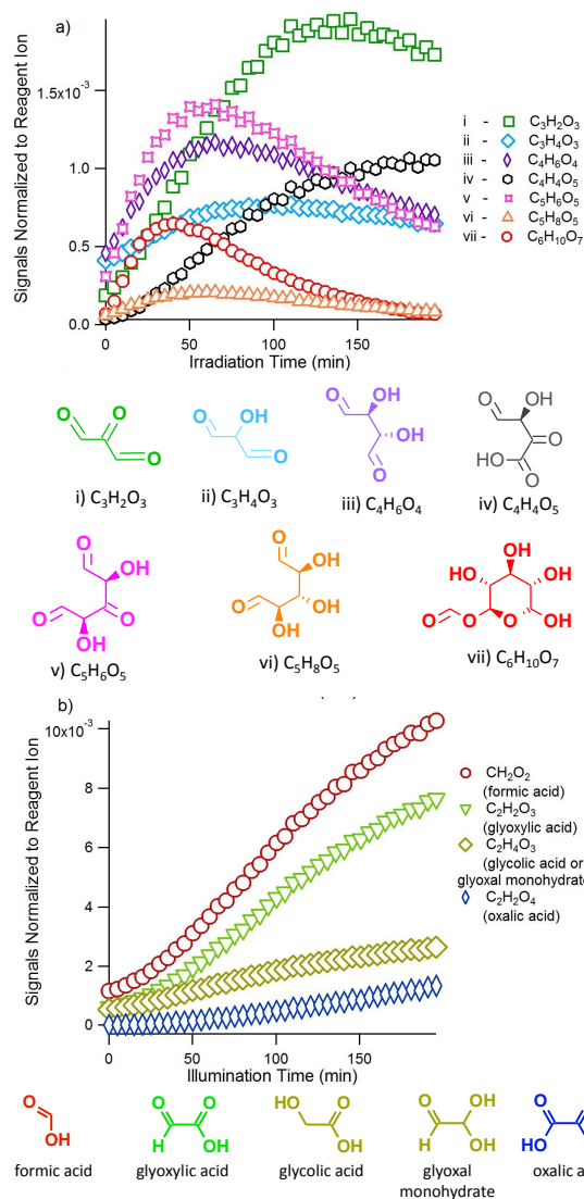
Fig. 5. Evolution of chain scission products measured by the I(H_2O)_n^- reagent ion. Selected major products with three to six carbons are shown in a), with their proposed structures. The proposed reaction mechanisms leading to their formation are attached in Supplementary Information Figure S1. Formation of small organic acids with one or two carbons are shown in b). All the signals have been normalized against the reagent ion ( I(H_2O)^- ) at m/z 145.
