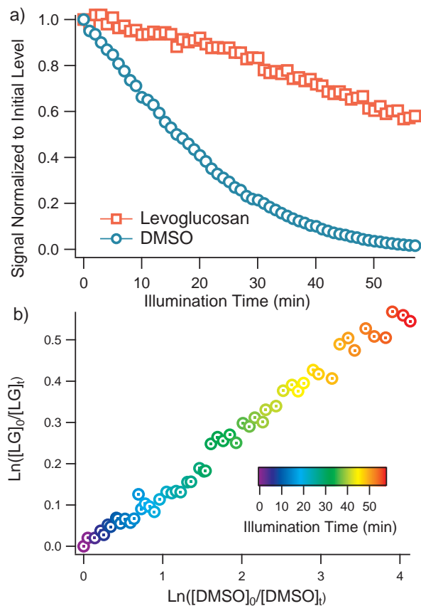
Fig. 9. The time series of LG and DMSO during a kinetic experiment (Exp. #1 in Table 1) are shown in (a). The signals are normalized to that at the beginning of the photooxidation. The relative kinetics plot from the same experiment is shown in (b) according to Eqn. 1. The color code indicates the illumination time.
