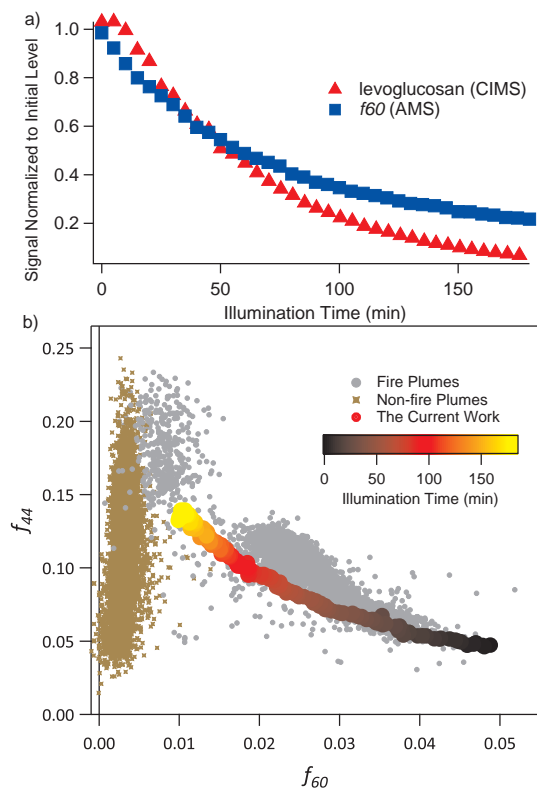
Fig. 10. The decay of levoglucosan monitored by the Aerosol-ToF-CIMS and the decay of f60 monitored by the AMS (a), and the f60 vs f44 trajectory from the current work compared to field measurements (b). The trajectory obtained in the current work is color coded with irradiation time. The compiled data (Cubison et al., 2011) from field measurements in fire plumes (grey) and non-fire plumes (brown) are also shown.
