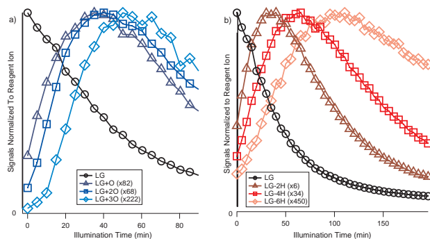
Fig. 2. The evolution of the +O (a) and the -2H (b) series from levoglucosan (LG). The signal of each compound normalized by the reagent ion intensity at m/z 145 ( I(H_2O)^+ ) is shown as a function of the irradiation time. The signals are multiplied by the bracketed number to be on scale.
