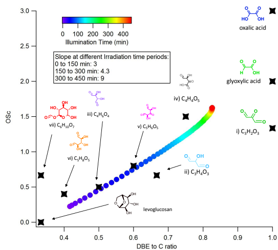
Fig. 7. OS_c vs DBE/C plot. The intensity-weighted average OS_c and DBE/#C from the products listed in Table S1 are displayed here. The color code represents the illumination time. The coordinates of major compounds are also shown.
