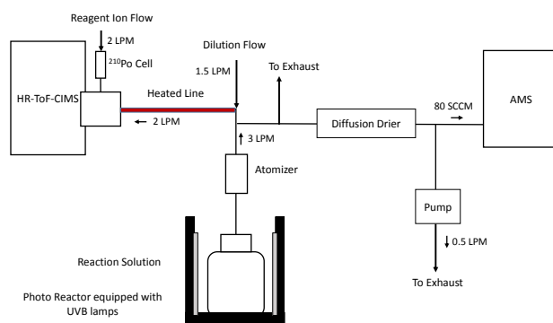
Fig. 1. The experimental apparatus.
