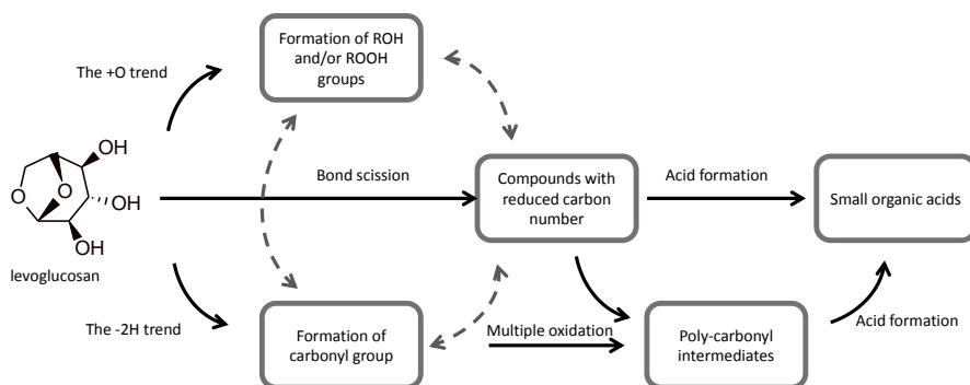
Fig. 8. A simplified overview of reaction mechanisms discussed in the current study. Solid arrows represent proposed reaction pathways of LG upon OH oxidation. The dashed arrows illustrate the complicity in the reaction system where each product can also take more than one reaction paths.
