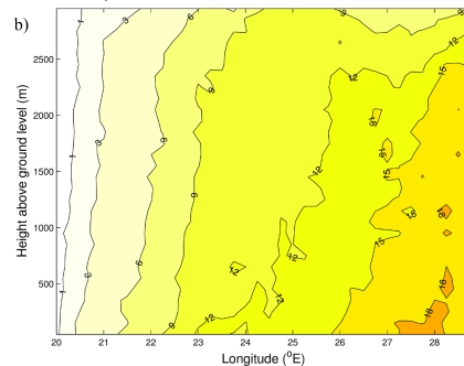
Fig. 6. (a) Dispersion model results from NAME for the mixing ratio of CH 4 originating from the local wetlands in a cross section of the atmosphere averaged over 67.75 to 68.00° N and 1 h surrounding 11:00 GMT on 22 July 2012. The local wetland CH 4 source was defined as a 1.2 mgCH 4 h -1 m -2 source emitted from the ground between 20 to 28° E and between 67 to 69.5° N. (b) shows the same but for a 1 h average surrounding 16:00 GMT on the same day.
