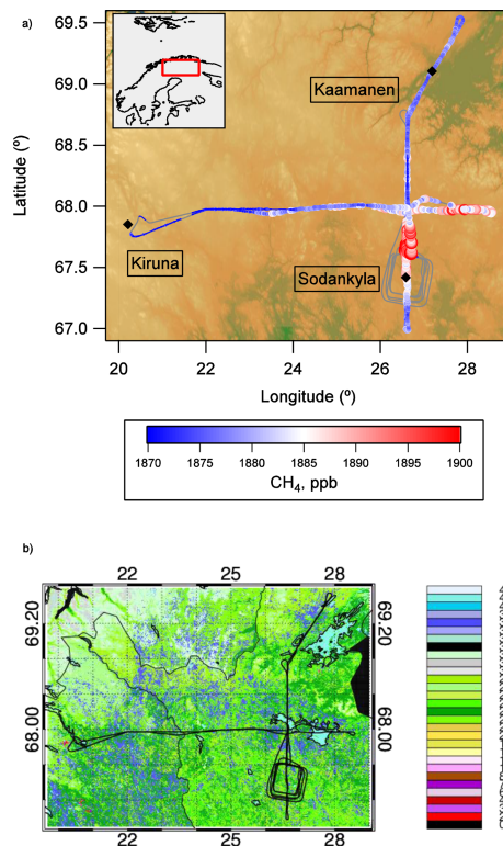
Fig. 1. (a) FAAM BAe-146 flight track for flight B720 (22 July 2012). Observations of \text{CH}_4 in the PBL are coloured according to the legend. Black diamonds mark Kiruna, Sodankylä and Kaamanen. (b) Flight track where the surface is coloured using the land use type (Corine land cover 2006). Numbers correspond to land types given in Table 1.
