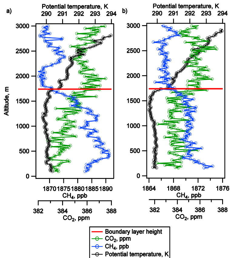
Fig. 4. (a) Ascending (01:00 GMT) and (b) descending (15:00 GMT) potential temperature profiles performed over Sodankylä during flight B720, used to determine the boundary layer height as described in the text.
