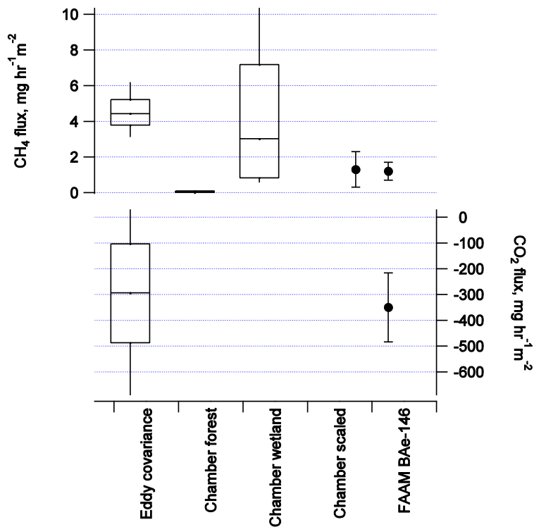
Fig. 5. A comparison between different techniques used to determine fluxes. The box extents define the 25th and 75th percentiles, and whiskers are the 10th and 90th percentiles. Note: the Eddy covariance percentiles are for daytime (06:00 to 18:00 GMT) only. Forest and wetland chamber fluxes represent summer seasonal statistics for 60 chamber measurements (21 in forest regions and 39 in wetland regions). The scaled chamber (black circle) is determined by averaging the wetland and forest chamber fluxes as described in Sect. 3.3. The FAAM BAe-146 and scaled chamber error bar shows the 1\sigma uncertainty as described in Sect. 3.1.
