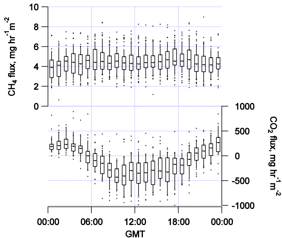
Fig. 7. CH 4 and CO 2 hourly fluxes at Sodankylä wetland site between 1 July and 15 August 2012 determined using the eddy covariance technique. CH 4 diurnal variation is noted to be small. Net CO 2 uptake occurs during the day, with net emission during the night.
