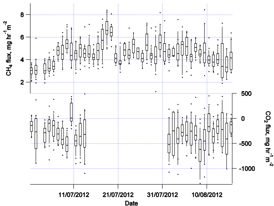
Fig. 8. Daytime (06:00–18:00) \text{CH}_4 and \text{CO}_2 fluxes at Sodankylä wetland site between 1 July and 15 August 2012 determined using the eddy covariance technique. Note: \text{CO}_2 fluxes are not shown for the period 14 July 2012 to 1 August 2012 as it was not possible to calibrate the LI-7200's \text{CO}_2 channel in that period.
