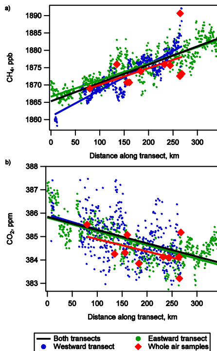
Fig. 3. (a) CH 4 and (b) CO 2 observations along a flight transect, which was aligned with the prevailing wind direction. The origin is 20° E, 68° N and the transect extends in an eastward direction. The gradients observed in both species were used to determine a net emission flux for the region using Eq. (3).
