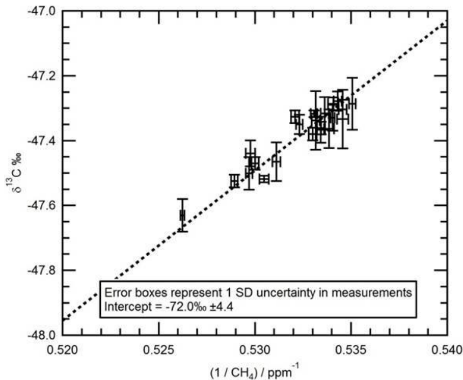
Fig. 2. Keeling plot showing PBL measurements of \delta^{13}\text{C}\text{-CH}_4 during flight on the 22 July 2012 (B720). The intercept of -72 \pm 4.4 \text{ ‰} is representative of a wetland source of \text{CH}_4 .
