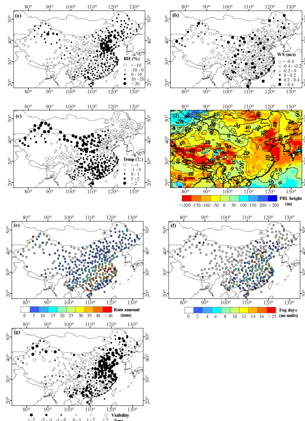
Fig. 3. The difference of (a) relative humidity, (b) wind speed, (c) temperature, (d) planetary boundary layer height (contour line represents the fraction of decreased PBL height in 2013 compared to previous years), and (g) visibility between January 2013 and the average values during the same period from 2007 to 2012. (e) The total precipitation amount and (f) total number of fog days in January 2013.
