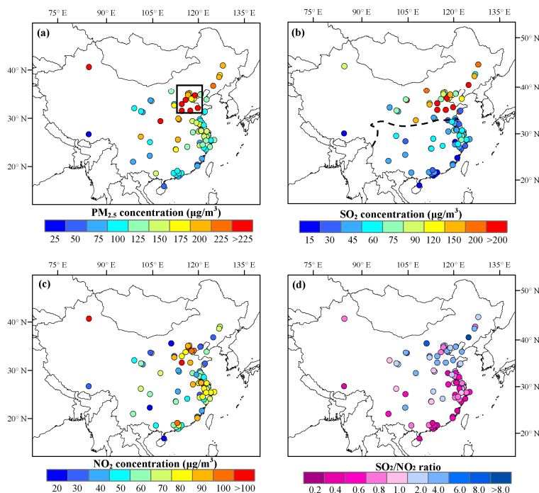
Fig. 2. The spatial distribution of mean concentrations of (a) PM 2.5 , (b) SO 2 , (c) NO 2 , and (d) the SO 2 /NO 2 ratios at 74 Chinese cities during January 2013. The Beijing-Tianjin-Hebei region is highlighted by the black rectangle in Fig. 2a. The dashed line in Fig. 2b represents the heating supply line that separates the northern heating region from the non-heating region (source: http://www.infzm.com/content/84193 , in Chinese).
