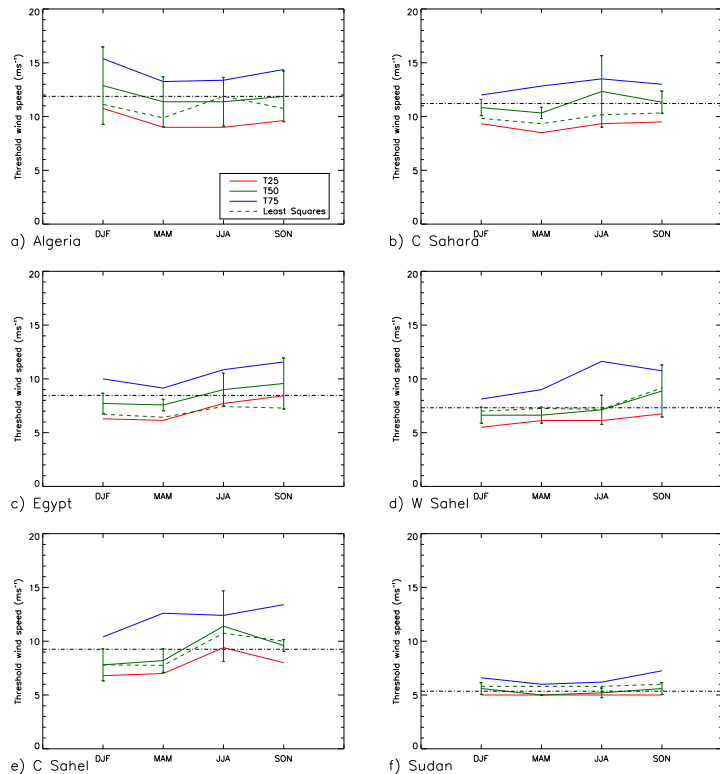
Figure 8. Seasonal threshold values averaged over six station groups (see Sect. 3.2.1 for definition): (a) N Algeria, (b) C Sahara, (c) Egypt, (d) W Sahel, (e) C Sahel and (f) Sudan according to the legend in the top left panel (for definition of thresholds, see Sect. 2.2.1). The dashed black lines indicate the annual mean T50. Seasons are December, January, February (DJF), March, April, May (MAM), June, July, August (JJA) and September, October, November (SON).
