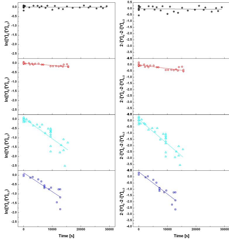
Fig. 4. Linearized plots for pseudo first order volume limited (left) and reacto-diffusion limited reaction (right): linearized plots for the reacto-diffusive case: 12 % RH (black stars, 3.2 \times 10^{-6} atm), 52 % RH (red circles, 6.1 \times 10^{-6} atm), 71 % RH (light blue triangles, 5.3 \times 10^{-6} atm) and 83 % RH (blue squares, 2.6 \times 10^{-6} atm). The slope of the linear fit equals the corresponding rate constant.
