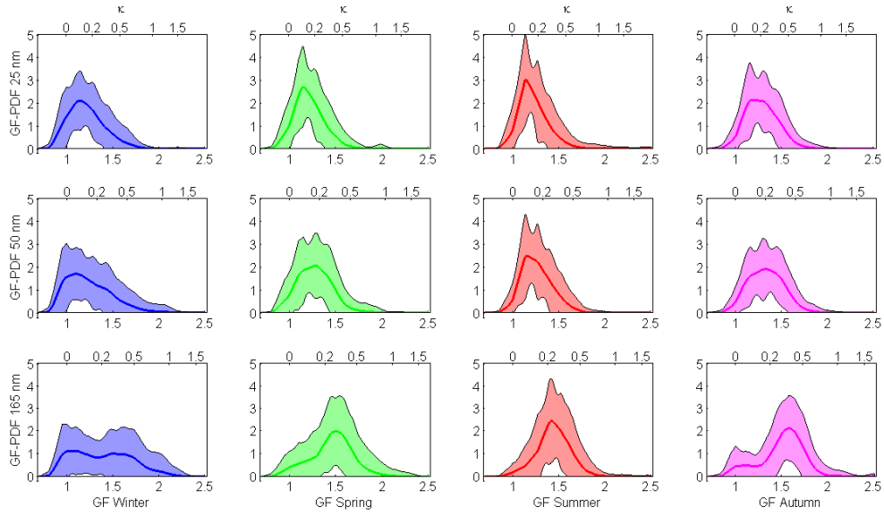
2 Figure 4a. Average GF-PDFs and their standard deviations for particles in the nucleation 3 mode (top panels), Aitken mode (middle panels) and accumulation mode (bottom panels), 4 split by season and measured at RH90. The bottom axis gives the growth factor GF and the 5 top axis shows the corresponding kappa value \kappa .
