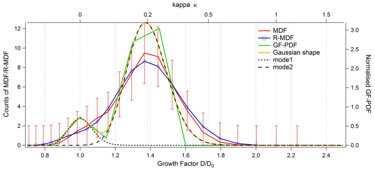
2 Figure 1. Example of a bimodal growth factor distribution function measured at RH90. The 3 red line refers to measured particle counts, i.e. the MDF (left axis), and the green line is the 4 GF-PDF (right axes). The black dotted lines and the yellow line are the results of super 5 positioning multiple Gaussians over the GF-PDF obtained from the TDMAinv program (right 6 axis). The bottom axis gives the growth factor GF and the top axis shows the corresponding 7 kappa value \kappa . Error bars indicate the estimated counting uncertainty of the measurements.
