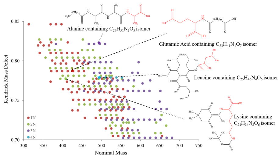
Fig. 7. Kendrick mass defect series ( CH_2 ) for CHON formulas containing 1–4 nitrogen atoms identified for samples N Am6 and N Am7 which make up the Primary Marine sample group. The molecular structures represent potential amino acid containing isomer compounds corresponding to several identified molecular formulas. The red portions of the molecular structures represent the amino acid portions of the compounds.
