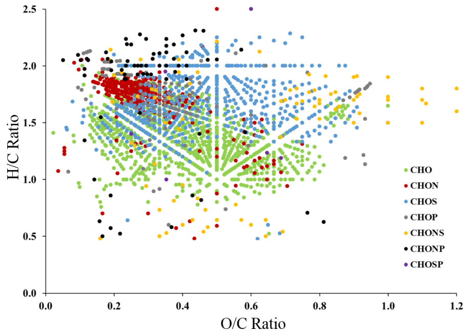
Fig. 4. van Krevelen diagram for the 2408 aerosol WSOM molecular formula input variables to the Principal Component Analysis. Data points are color coded for molecular formula elemental composition as described in the figure key.
