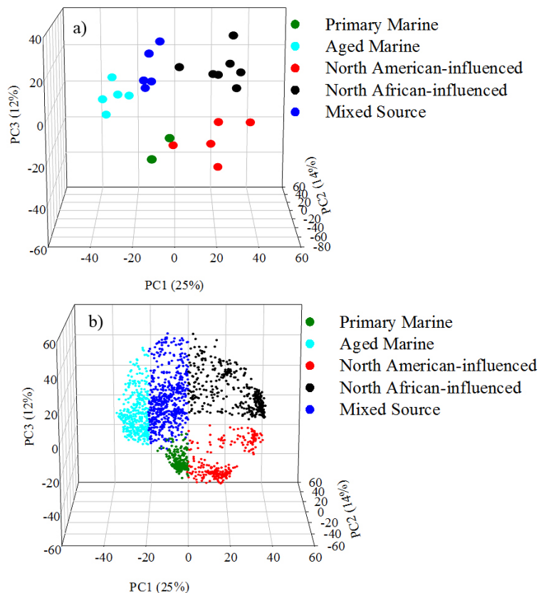
Fig. 5. Three dimensional plots showing the (a) sample scores and (b) variable (molecular formulas) loadings for the first three principal components accounting for 51 % of the variance in the dataset. Sample data points with similar PC scores are color coded for classification of samples into sample groups with similar molecular characteristics. The loadings assumed to be important components of each group are similarly color coded.
