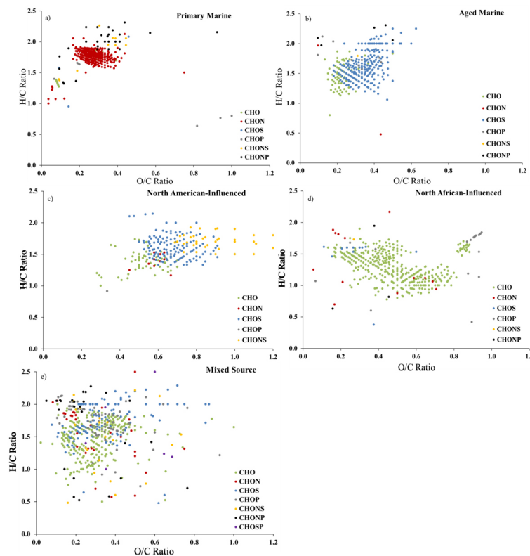
Fig. 6. van Krevelen diagrams corresponding to the WSOM loadings for the sample groups assigned by the PCA and classified as (a) Primary Marine, (b) Aged Marine, (c) North American-Influenced, (d) North African-Influenced, and (e) Mixed Source samples. Data points are color coded for molecular formula elemental composition as described in the figure key.
