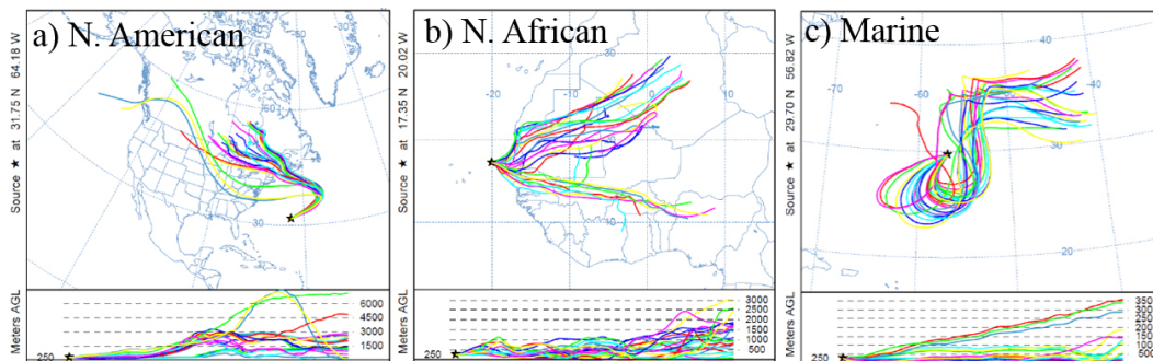
Fig. 2. Representative ensemble air mass back trajectories for samples influenced by (a) North American, (b) North African, and (c) Marine (minimal recent continental influence) air masses.
