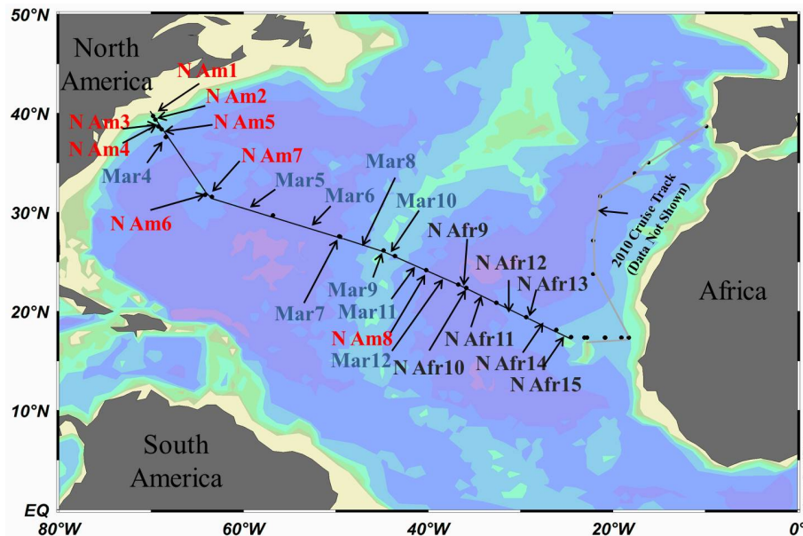
Fig. 1. Aerosol particulate collection locations during the 2011 US GEOTRACES cruise. Arrows pointing to a dot were collected on station. Arrows pointing to the line were collected in transit. Samples labeled as “N Am”, and “N Afr” showed a majority of 5 day ensemble air mass back trajectories extending back to the North American and African continents. Samples labeled “Mar” showed 5 day ensemble air mass back trajectories that had minimal continental influence.
