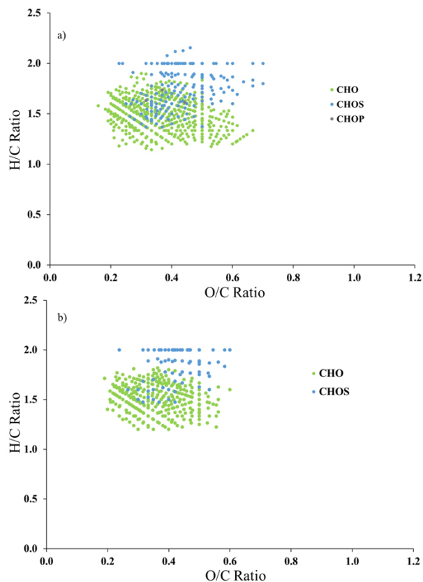
Fig. 3. van Krevelen diagrams for aerosol WSOM molecular formulas assigned to greater than (a) 75 % (at least 18 samples) and (b) 90 % (at least 22 samples) of the 24 aerosol samples. Data points are color coded for molecular formula elemental composition as described in the figure key.
