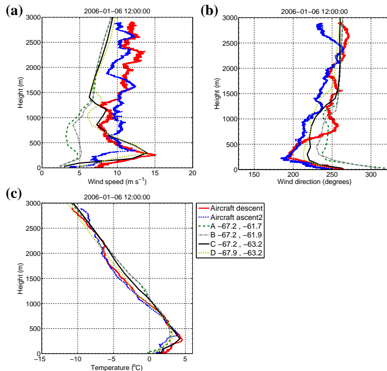
Fig. 5. Profiles from the aircraft observations and from domain 3 of the WRF model. Aircraft profiles were taken during the descent down to the ice shelf between 20:14 and 20:24 UTC on 6 January and during the ascent away from the ice shelf before the journey back to base from 22:00 to 22:09 UTC. Model profiles are for 12:00 UTC on 6 January from various locations (labeled with letters in the legend). See Fig. 7b for a map of the locations of these profiles. The profiles are: (a) wind speed, (b) wind direction and (c) temperature.
