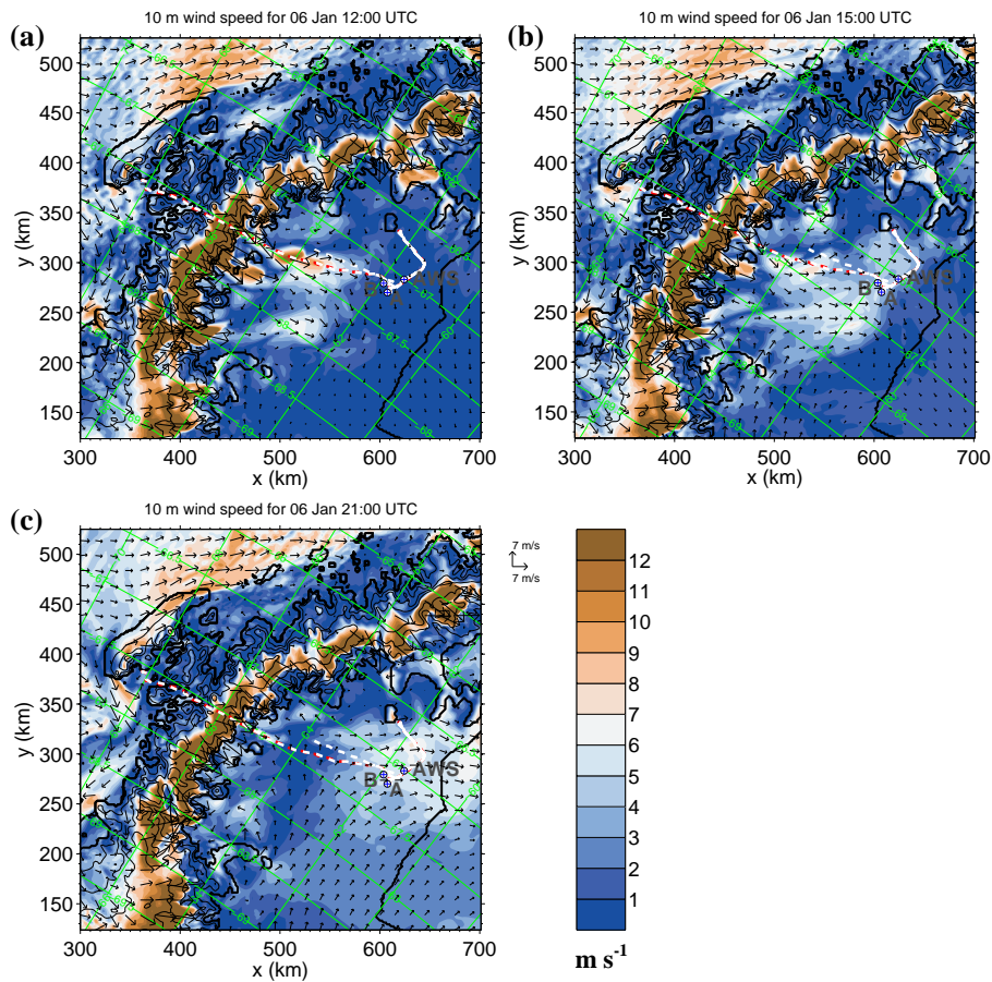
Fig. 13. 10 m wind speeds (colours and vectors) for 6 January at (a) 12:00 UTC, (b) 15:00 UTC and (c) 21:00 UTC.
