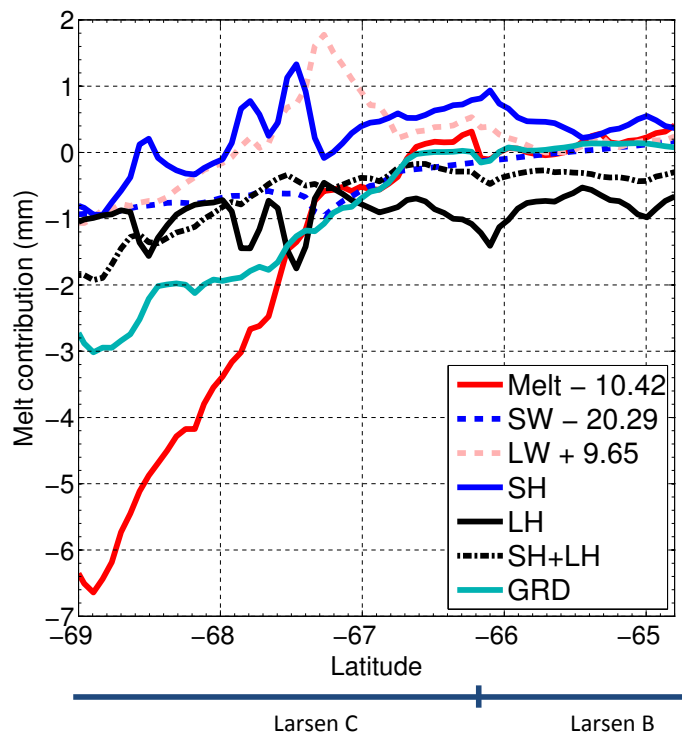
Fig. 19. Simulated total melting amount averaged along lines of constant latitude across the Larsen Ice Shelf (“Melt”) for the times of 12:00, 15:00, 18:00 and 21:00 UTC on 6 January. Also shown are the net contributions to the surface melting (i.e. positive values indicate a net downward contribution) at these times from shortwave radiation (“SW”), longwave radiation (“LW”), sensible heat flux (“SH”), latent heat flux (“LH”), combined sensible and latent heat flux (“SH + LH”) and ground flux (“GRD”). The lines “Melt”, “SW” and “LW” have been shifted by -19.8 , -27.7 , and +7.6 mm respectively in order to make all the lines visible on the same plot. These shifts were designed to make the values zero at the Larsen B reference location at 65.6^\circ S. The approximate boundary between Larsen B and Larsen C is also marked.
