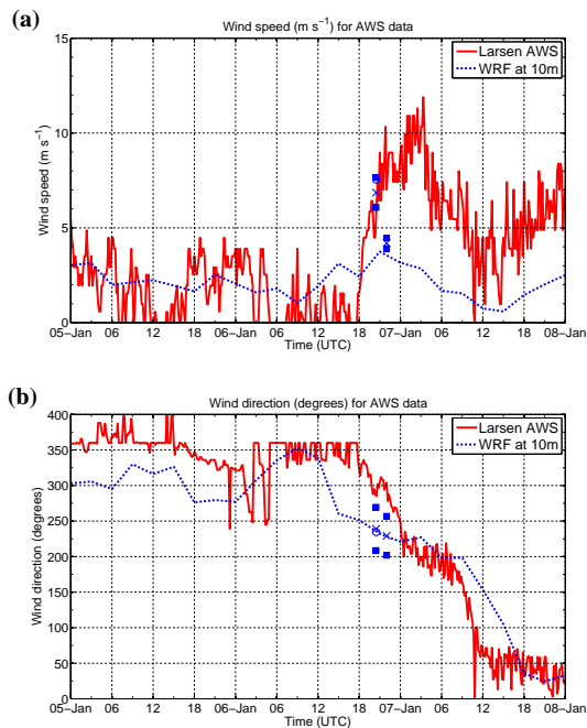
Fig. 12. Timeseries from the Larsen C AWS along with the modeled values at the AWS location in domain 3; (a) 10 m wind speed ( S ) and (b) 10 m wind direction ( \phi ). Also marked are details of aircraft observations made during the A–L1 leg at 15 m altitude. For S the mean values are shown by the blue cross and the filled squares denote \pm 1\sigma . For \phi the squares denote the full range of the wind direction during the leg and the cross shows the midpoint of the range. The circles show the observed value when the aircraft was directly above the AWS location. The same is marked for the later descent towards the ice shelf just before the final ascent from the region.
