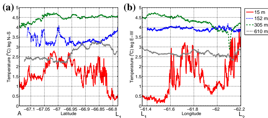
Fig. 11. As for Fig. 10 except for temperature and with no smoothing.
