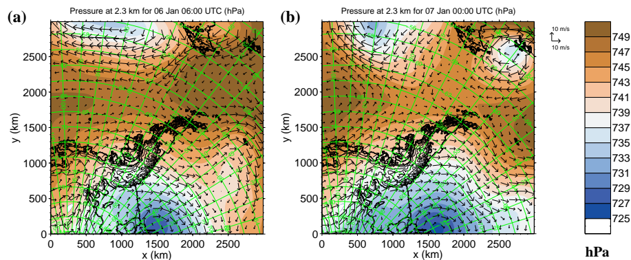
Fig. 2. Pressure and wind vectors at 2.3 km a.s.l. for WRF domain 2 at (a) 6 UTC on 6 January and (b) 0 UTC on 7 January.
