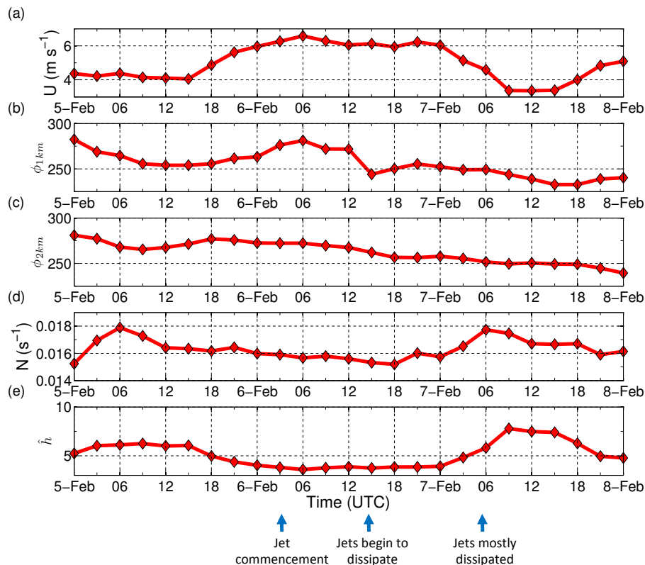
Fig. 17. Timeseries of various quantities taken from the profile at the lefthand edge of the cross section in Fig. 15. (a) shows the component horizontal wind for the cross section averaged between heights of 0 and 2 km; (b) and (c) show the wind direction ( \phi ) at heights of 1 and 2 km, respectively; (d) shows that Brunt Väisälä frequency; and (e) shows the non-dimensional mountain height. Also marked are notable times for the development of the near surface jet along Larsen C.
