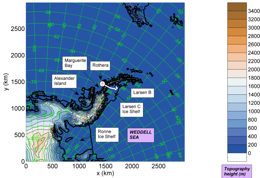
Fig. 3. The area of the second WRF domain (see Fig. 1) showing the topography height (coloured contours) and various landmarks, including the Rothera BAS research base (white dot with red cross inside). The aircraft flight track is indicated by a white line.
