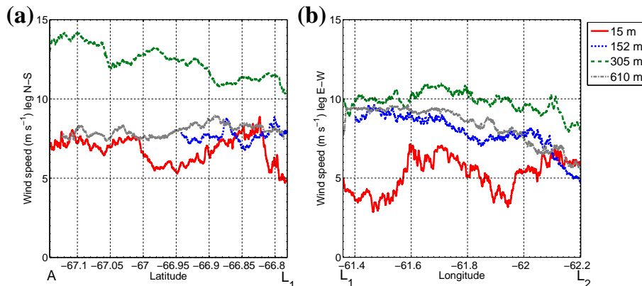
Fig. 10. Wind speed during the “L” shaped legs flown from A to L1 to L2 at the heights indicated. See Fig. 7d for the position of these locations. The A–L1 leg was orientated close to south-north and the L1–L2 leg close to east-west. Thus, the x-axis was chosen to be latitude for the A–L1 leg (a) and longitude for the L1–L2 leg (b) . Also, here the data has been smoothed over 3 s windows for clarity. Note, part of the N–S leg at 152 m in (a) has been removed due to wind measurement problems caused by a loss of GPS lock.
