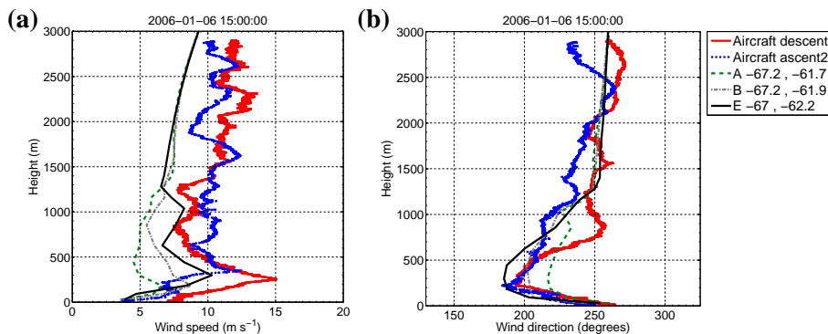
Fig. 9. As for Fig. 5 except for at 15:00 UTC on 6 January and for wind speed (a) and direction (b) only. See Fig. 7c for a map of the locations of these profiles.
