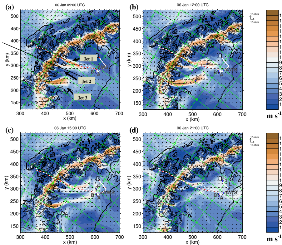
Fig. 7. As for Fig. 6 except in close up view over the ice shelf and at different times on 6 January: 09:00 UTC (a) , 12:00 UTC (b) , 15:00 UTC (c) and 21:00 UTC (d) . Also marked are the locations of various other points where the model profiles in Figs. 5 and 9 have been taken.
