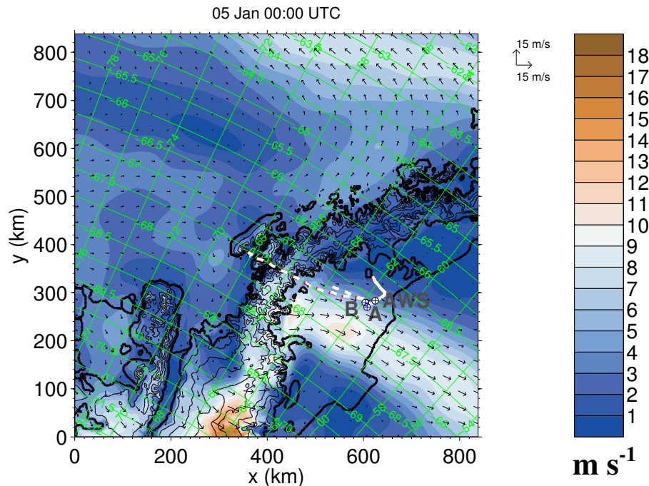
Fig. 6. Domain 3 horizontal wind speed and wind vectors on the 4th vertical model level at the beginning of the simulation at 00:00 UTC for 5 January 2006. This therefore represents the initial wind field as interpolated from the ECWMF analysis. Marked on here is the flight path of the aircraft (white dotted line). The marked location, A, is where the maximum wind speed was measured during the aircraft's descent onto the ice shelf. Location B is the position of the maximum wind speed during the ascent from the ice shelf before flying back over the peninsula. Also marked is the location of the Automatic Weather Station (AWS).
