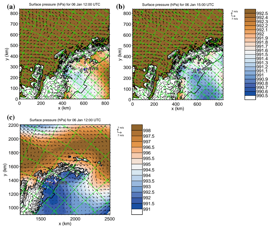
Fig. 14. Surface pressure (colors; hPa) and 10 m wind vectors for 6 January. (a) and (b) show WRF domain 3 at 12:00 and 15:00 UTC, respectively, and (c) shows a close up of domain 2 at 12:00 UTC.
