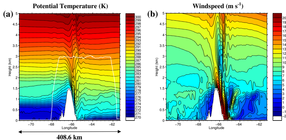
Fig. 15. Vertical cross sections of potential temperature (a) and horizontal component wind speed (b) along the straight line in Fig. 7a for 09:00 UTC on 6 Jan. The white solid line in (a) shows the height of the aircraft projected onto the longitude of the cross section.
