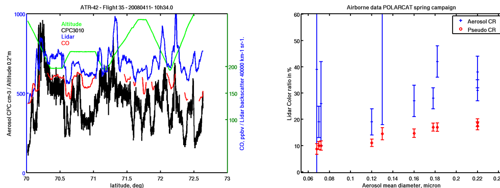
Fig. 3. (left) Comparison of lidar attenuated backscatter 120 m to 200 m below the aircraft in relative units with in-situ measurements of CO (red) in ppbv, and aerosol concentration (black) in particles per \text{cm}^{-3} for a flight (35) with crossing of several aerosol layers. Green curve is the aircraft altitude in 5 m unit. (right) Lidar color ratios (pseudo CR for total backscatter and aerosol CR for aerosol backscatter) in % for 10 aerosol layers where in-situ and lidar data can be compared (see Table 2) vs. the SMPS aerosol mean diameter.
