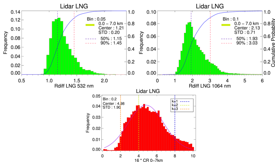
Fig. 2. Distribution and cumulative probability (blue) of the 532 nm (left), 1064 nm (middle) backscatter ratios measured by the airborne lidar from 30 March to 11 April. Mean, standard deviation, median and 90th percentile are given for each distribution. The distribution of the aerosol color ratio CR_a \times 16 (right panel) is compared to the lines for CR_a = 0.125 ( k = 3 ), CR_a = 0.25 ( k = 2 ) or CR_a = 0.5 ( k = 1 ).
