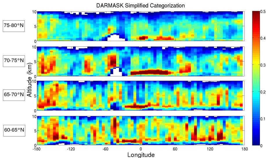
Fig. 15. Zonal vertical cross sections of the cloud fraction derived from the DARDAR products for April 2008 in 4 latitude bands from 60° N to 80° N. The longitudinal resolution is 5° and the vertical resolution is 60 m.
