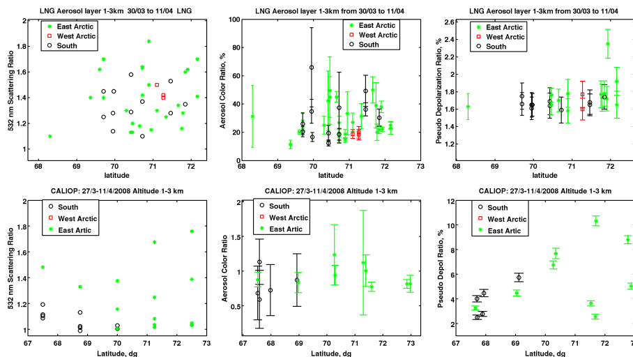
Fig. 9. Latitudinal distribution of 532 nm backscatter ratio, aerosol color ratio and pseudo depolarization ratio for the airborne lidar observations (top) and filtered level 1 CALIOP (bottom) at altitudes < 3 km during the aircraft campaign. The colors are for different air mass origins estimated with Flexpart (see text).
