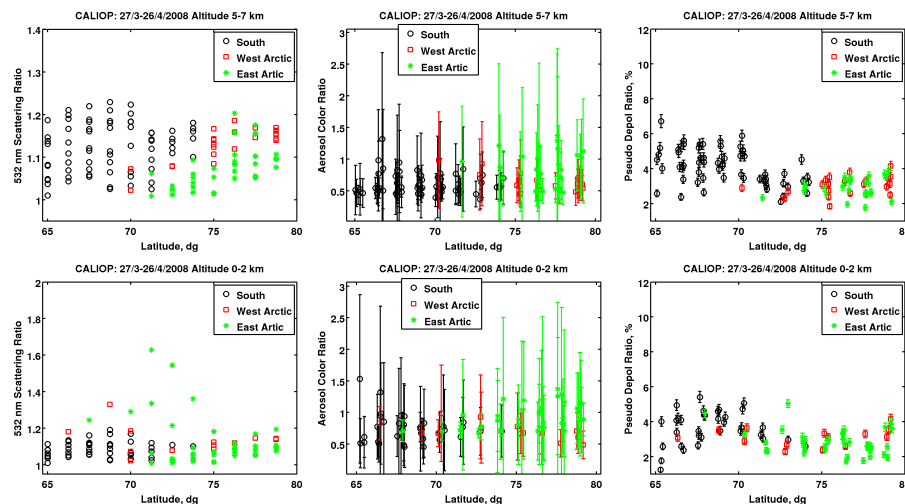
Fig. 12. Latitudinal distribution of 532 nm backscatter ratio, aerosol color ratio and pseudo depolarization ratio for filtered level 1 CALIOP in April 2008 at altitudes < 2 km (bottom) and between 5 km and 7 km (top). The origin of the layers are estimated with Flexpart (see text).
