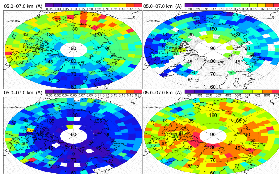
Fig. 14. Map of the 532 nm backscatter ratio, aerosol color ratio, pseudo depolarization ratio and fraction of cloudless observations using the April 2008 filtered level 1 CALIOP data in the 5–7 km altitude range.
