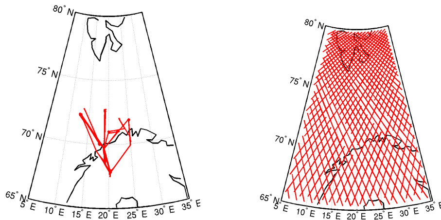
Fig. 1. Aircraft trajectories for the measurement days listed in Table 1 (left) and positions of the CALIOP tracks from 27 March to 11 April (right).
