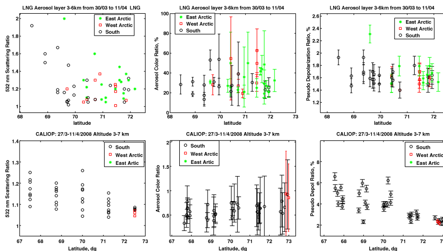
Fig. 10. Latitudinal distribution of 532 nm backscatter ratio, aerosol color ratio and pseudo depolarization ratio for the airborne lidar observations (top) and filtered level 1 CALIOP (bottom) at altitudes between 3 km and 7 km during the aircraft campaign. The colors are for different air mass origins estimated with Flexpart (see text).
