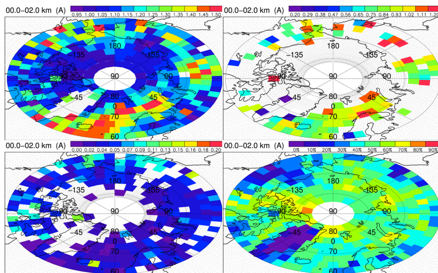
Fig. 13. Map of the 532 nm backscatter ratio, aerosol color ratio, pseudo depolarization ratio and fraction of cloudless observations using the April 2008 filtered level 1 CALIOP data in the 0–2 km altitude range.
