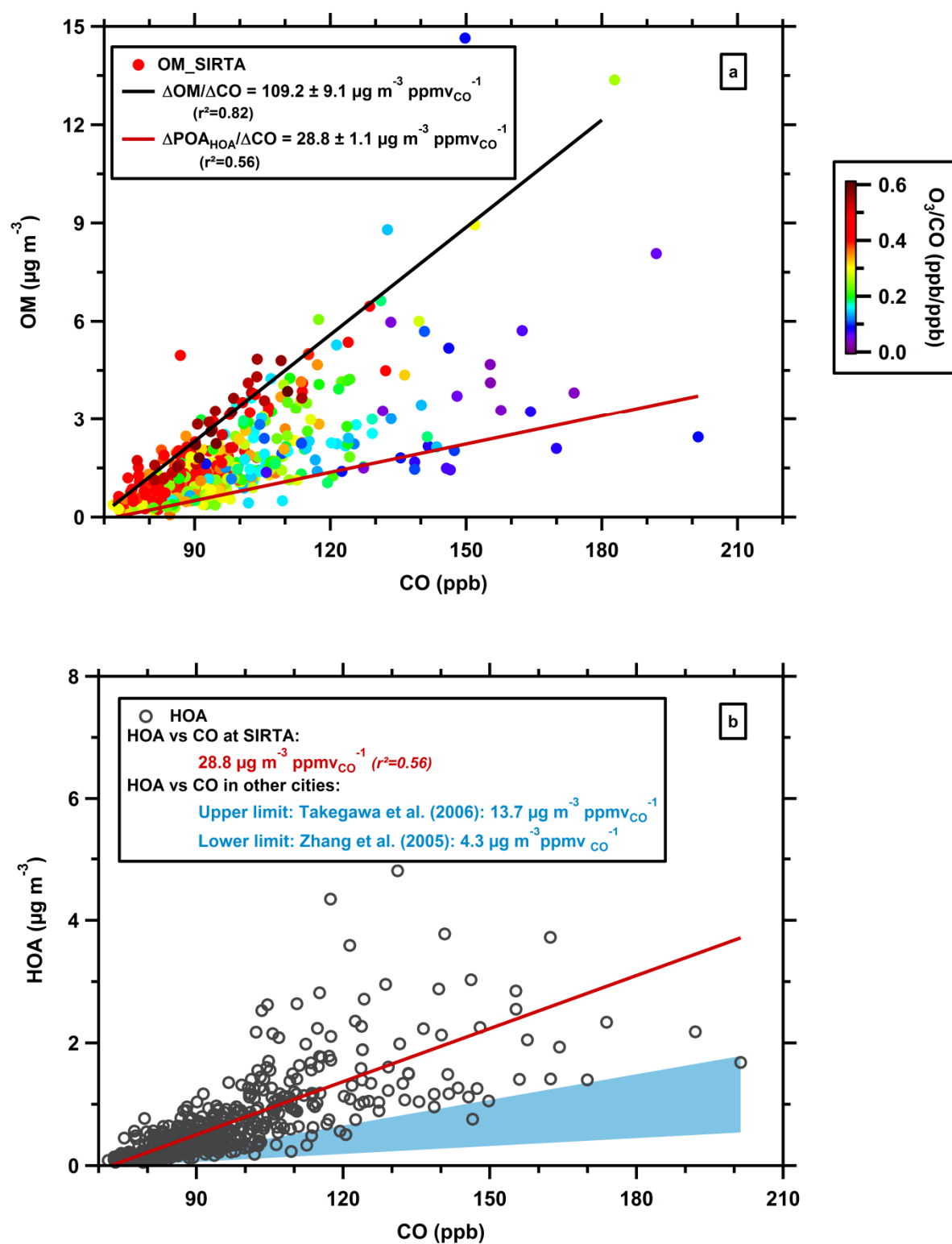
Figure 5. Scatterplots of OM versus CO (a) and scatterplots of HOA versus CO (b) in suburban Paris in summer 2009. OM, CO and HOA were averaged to 1 hour.
