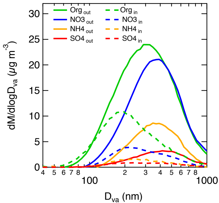
Fig. 5. Mass size distribution of major constituents of submicron particle out-of-fog (straight line) and in fog (dotted line) averaged over the entire campaign.
