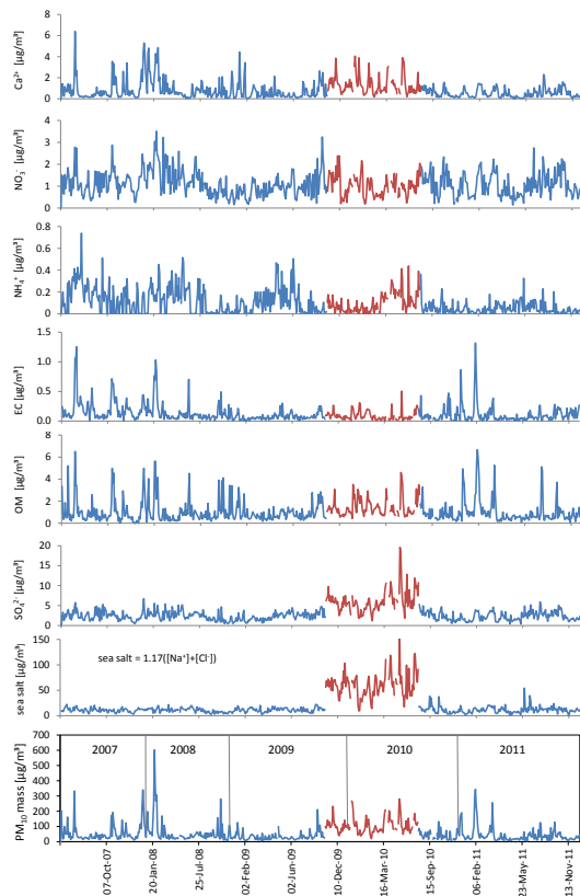
Fig. 3. Time series of mass concentration and major PM_{10} aerosol components in filter samples collected during the five years from 2007 to 2011. During the period from 23 October 2009 till 9 July 2010 (red line) all samples were collected on top of a storage container with an inlet height of 4 m above ground, all other samples were collected on top of the tower with an inlet height of 32 m above ground.
