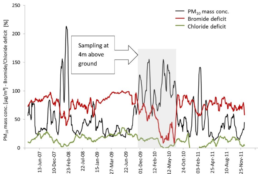
Fig. 9. Variability of bromide and chloride deficit in comparison to the total \text{PM}_{10} mass concentration (all curves represent 10-samples running means) and the season.
