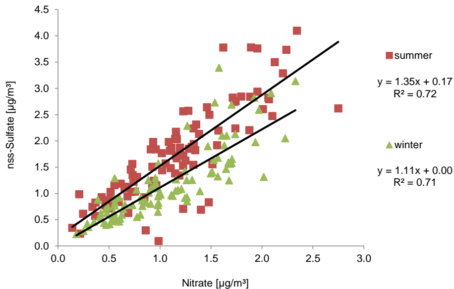
Fig. 5. Correlation between nitrate and nss-sulfate between summer and winter in samples collected from July 2010 to November 2011.
