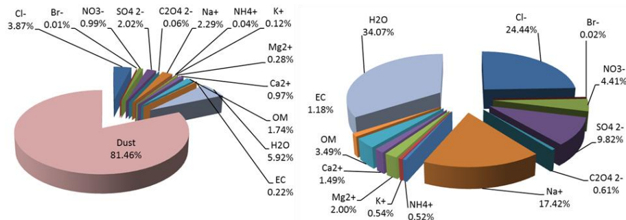
Fig. 2. Averaged PM constitution for 49 mineral dust dominated aerosol samples (left) and 183 marine samples (right) collected at 32 m on top of the tower.
