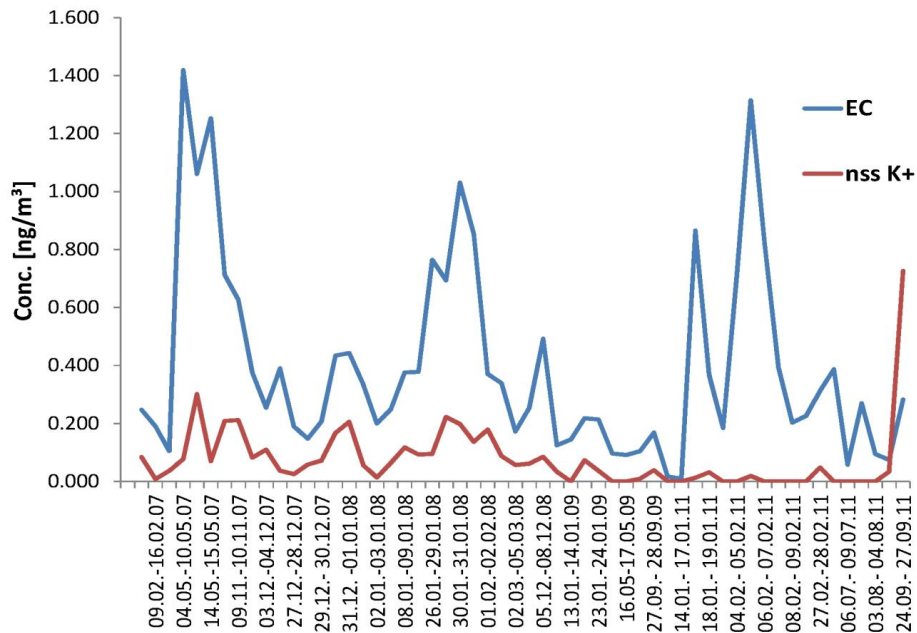
Fig. 8. Time series of nss-potassium (nss-K + ) and elemental carbon (EC) measured during air mass inflow from Africa revealing similar temporal variations.
