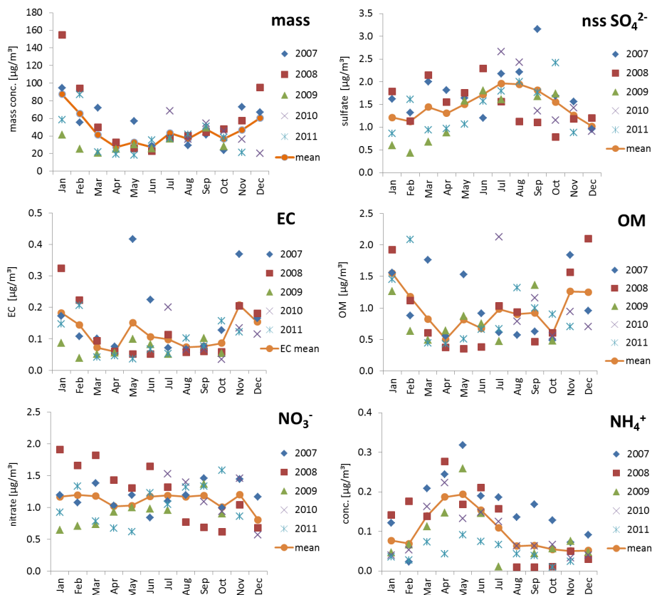
Fig. 4. Annual variability and monthly mean of \text{PM}_{10} mass concentration, non-sea-salt sulfate, elemental carbon (EC), organic matter (OM), nitrate, and ammonium during the five years of measurements for samples collected on the tower.
