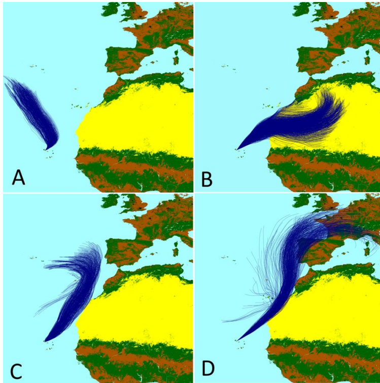
Fig. 1. Typical air mass back trajectories observed at CVAO during the routine filter sampling periods, aerosol type and PM_{10} mass concentration are given in parentheses: (A) 2 May 2011: Northern Atlantic Ocean (pure marine air mass, m = 8.28 \mu\text{g m}^{-3} ); (B) 14 January 2011: Saharan air mass (dust loaded, m = 155.04 \mu\text{g m}^{-3} ); (C) 2 February 2011: Air mass from Europe crossing the coast-line of NW Africa and the Canary Islands (anthropogenically influenced, m = 64.89 \mu\text{g m}^{-3} ); (D) 12 July 2008: Marine air (slightly polluted from the Northwest-African coast and the Canary Islands, m = 21.61 \mu\text{g m}^{-3} ).
