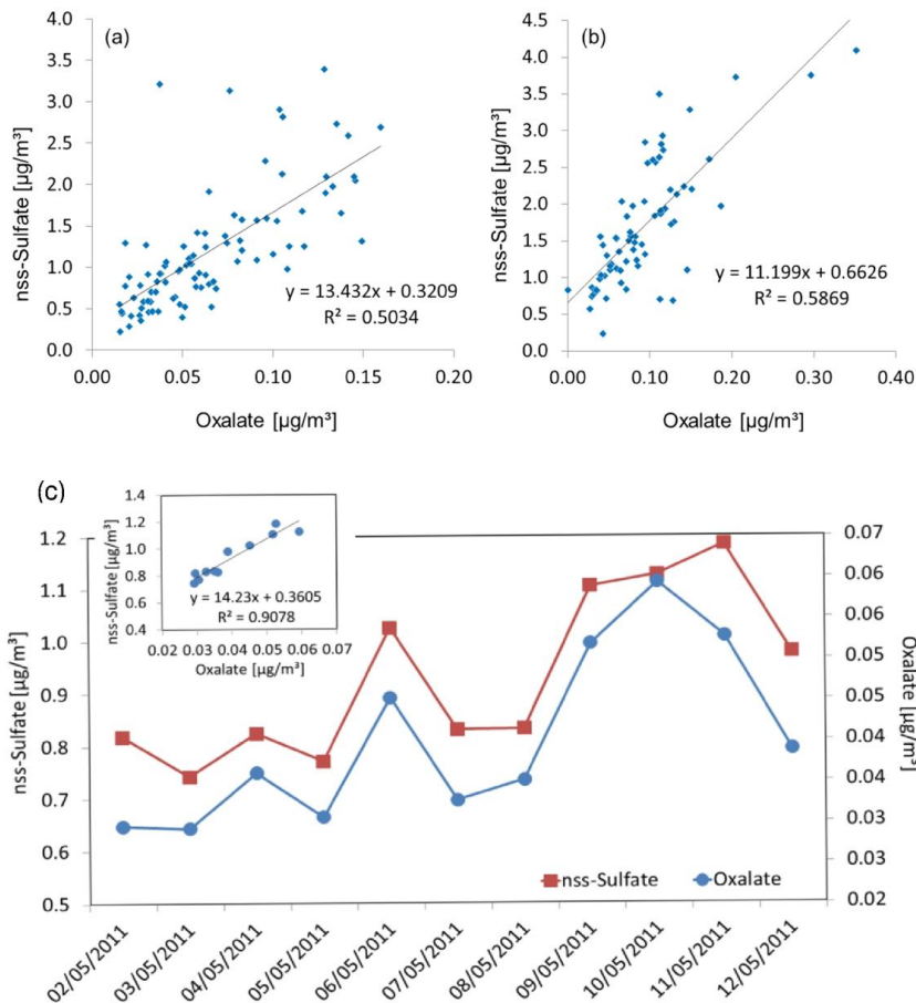
Fig. 6. Correlation between nss-sulfate and oxalate in filter samples during 2010/2011, above (a) winter, (b) summer, and below concentration and correlation during a marine clean air episode in May 2011.
