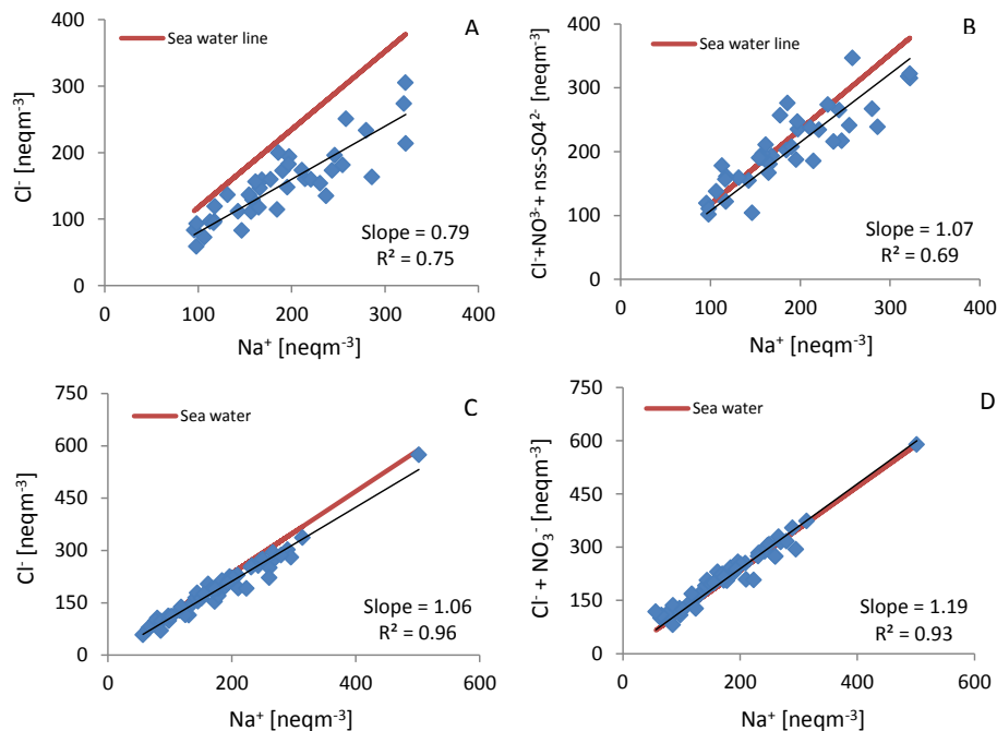
Fig. 10. Scatter plots between (A) \text{Na}^+ and \text{Cl}^- , (B) \text{Na}^+ and \text{Cl}^- + \text{NO}_3^- + \text{nss-SO}_4^{2-} during summer marine air mass inflow and (C) \text{Na}^+ and \text{Cl}^- , (D) \text{Na}^+ and \text{Cl}^- + \text{NO}_3^- during Saharan dust events at the CVAO.
