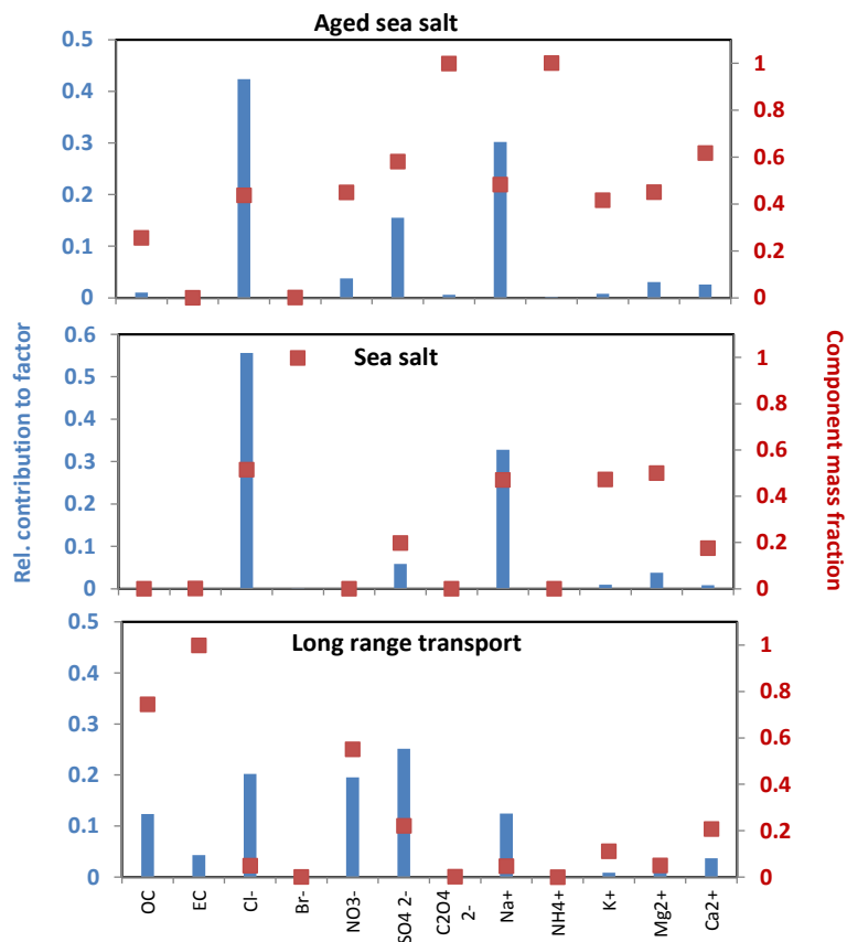
Fig. 11. Source profiles identified from measured PM 10 components at CVAO. Results are from 671 analyzed filters. The relative contribution of each species to a given factor is represent as blue bars while the relative contribution of each factor to the total specie concentration is represented as red square (right axis).
