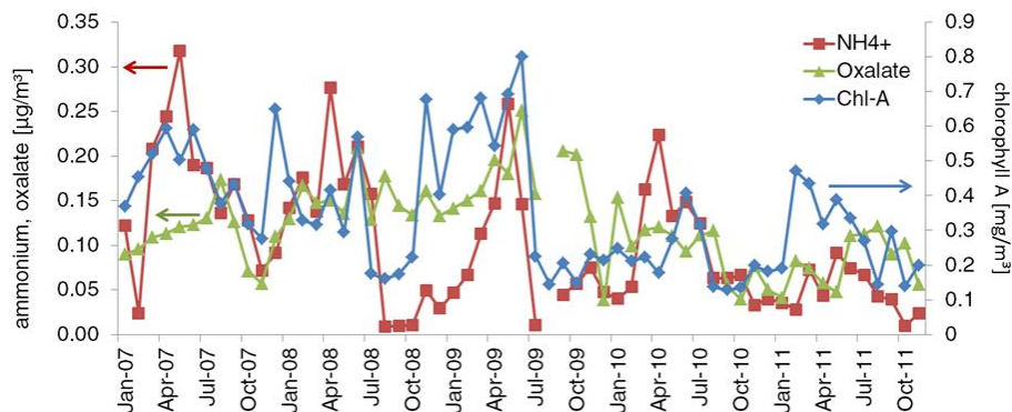
Fig. 7. Monthly mean of chlorophyll a in the tropical NE Atlantic (selected area for averaging: Lat (16.985, 24.895), Lon (−24.87, −18.278)), oxalate and ammonium in PM 10 aerosol samples collected at the CVAO.
