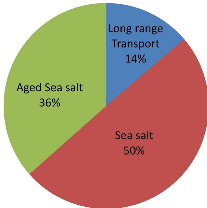
Fig. 12. Average contribution of each source to the total analyzed species.
