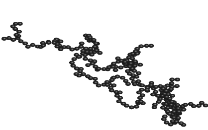
(a) D_f = 1.5
