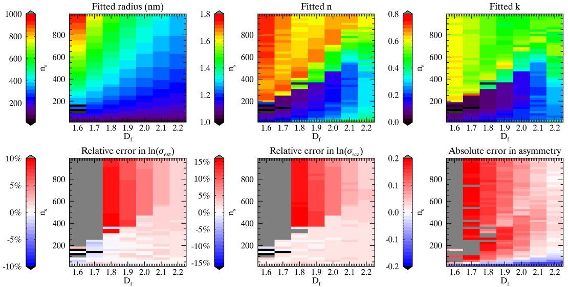
Fig. 8. The optimum fitted sphere parameters ( r , n , and k ) and their resultant errors relative to the reference MSTM calculations in \ln\sigma_{\text{ext}} , \ln\sigma_{\text{sca}} and absolute errors in g for BCFA with \lambda = 550 nm. The colour scale has been adjusted so that the very large errors caused by unphysically small BCFA D_f are clipped.
