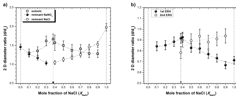
Figure 6. (a) 2-D diameter ratios ( d/d_x ) of the particles/aerosols plotted as a function of the NaCl mole fractions ( X_{NaCl} ), which represent the size increase due to the mutual deliquescence of the eutonic part at MDRH ( d_x ) compared to that of the solid particle at the start of the first transition ( d_x ) (eutonic: open squares); and due to the complete deliquescence of the remnant salts (in the figure, NaNO 3 : closed circles and NaCl: open circles) at their second DRHs ( d_x ) compared to that of the partially deliquesced particle at MDRH ( d_x ) and (b) 2-D diameter ratios ( d/d_x ) of droplets/aerosols plotted as a function of the NaCl mole fractions ( X_{NaCl} ), which represent the size decrease due to the efflorescence of NaCl ( d_x ) compared to that of the liquid droplets at the start of the first efflorescence ( d_x ) (first ERH: closed circles); and due to the mutual efflorescence of the remnant eutonic compositions (second ERH: open circles) ( d_x ) compared to that of the partially effloresced particles ( d_x ).
