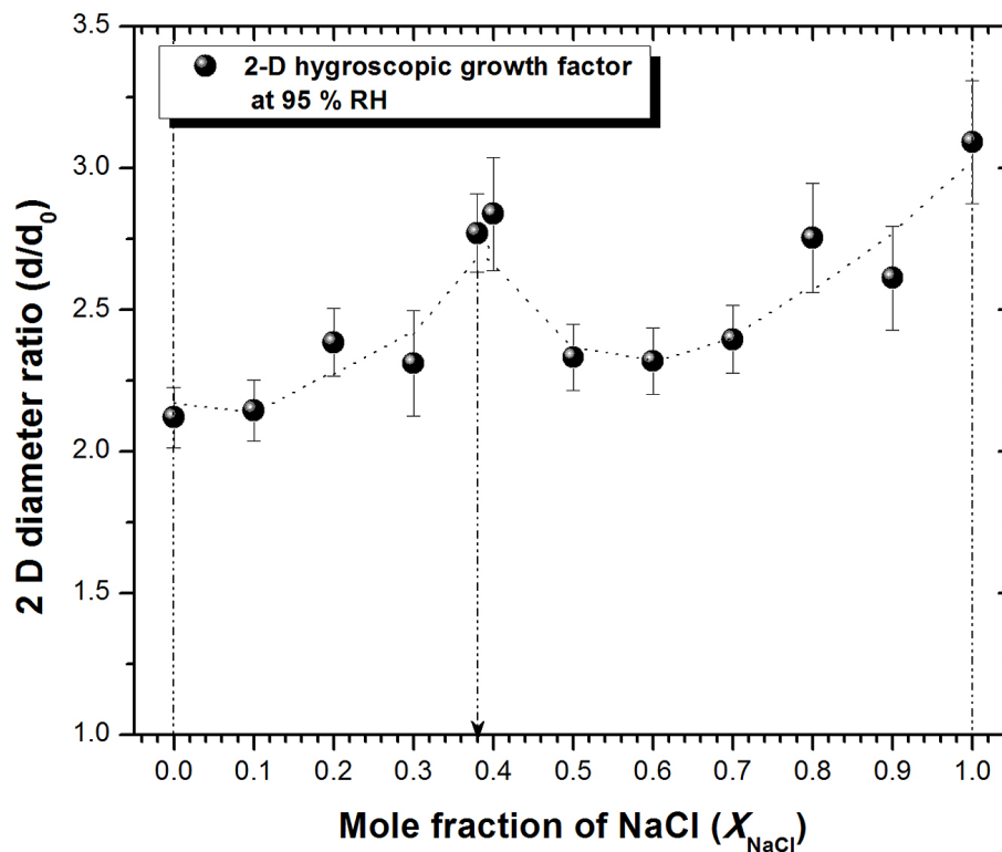
Figure 7. Hygroscopic growth factors in terms of the 2-D diameter ratios ( d_{95}/d_0 , where d_{95} \equiv the diameter at \sim 95\% , determined by extrapolation, and d_0 \equiv dry diameter at lowest or \sim 3\% RH) are plotted as a function of the mole fraction of NaCl for the NaCl-NaNO 3 mixture particles.
