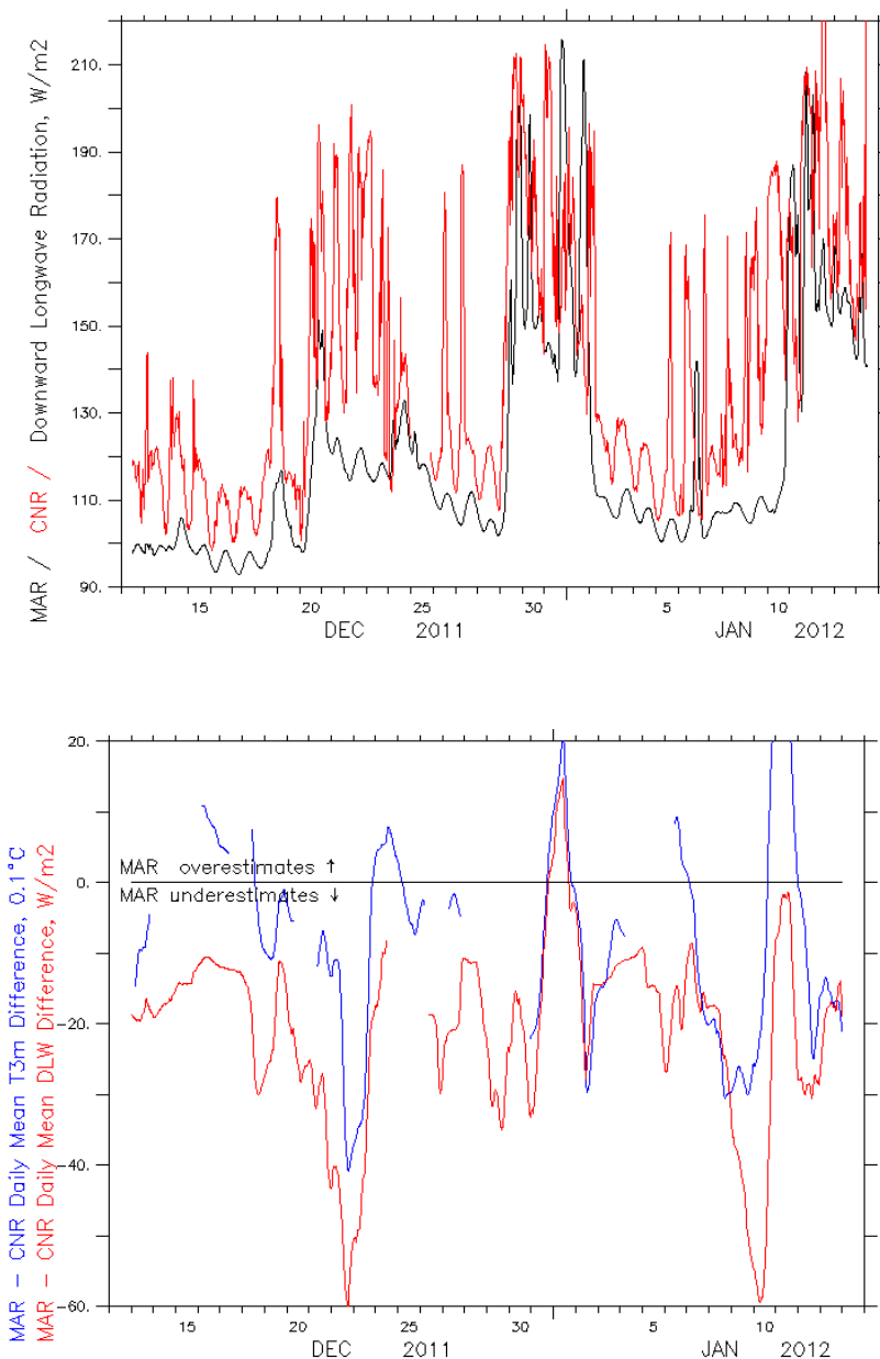
765 Fig. 2. Top : Long-wave Downward radiation (LWD, W/m^2 ) : simulation (dark line) and observation (red line). Data were averaged over an interval of 30 minutes. Bottom : comparison between the daily averaged LWD bias (red line) and air temperature bias (blue line, units : 0.1^\circ C ). Observations are those of the ISAC. MAR temperatures are averaged between 2 m and 4 m a.g.l. Gaps correspond to the absence of observations.
