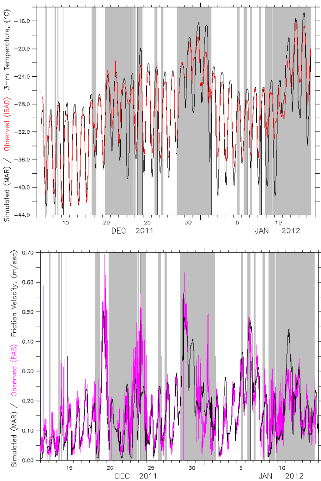
805 Fig. 3. Simulation (dark line) of wind speed (top left), wind direction (top right), and air temperature (bottom left) at Dome C, 3 m a.s.l., compared with ISAC observations. Bottom right: simulation of friction velocity (dark line) compared with BAS observations (magenta line). Data were averaged over an interval of 30 minutes. Shaded area indicate periods with DLW > 130 -2 Wm
