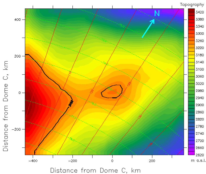
Fig. 1. The MAR integration domain and topography. The solid line refers to the 3250 m isocontour.
