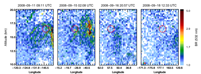
Figure 4. CALIOP Backscatter Ratio (colour coded) vs altitude and longitude. Red circles highlight the intersection with the 400K isentropic trajectory.
