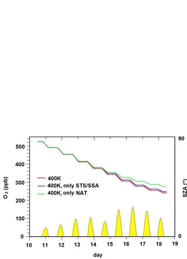
Figure 8. O 3 evolution taking into account the full heterogeneous chemistry (red), or going on only on NAT (green) or on STS/SSA (blue).
