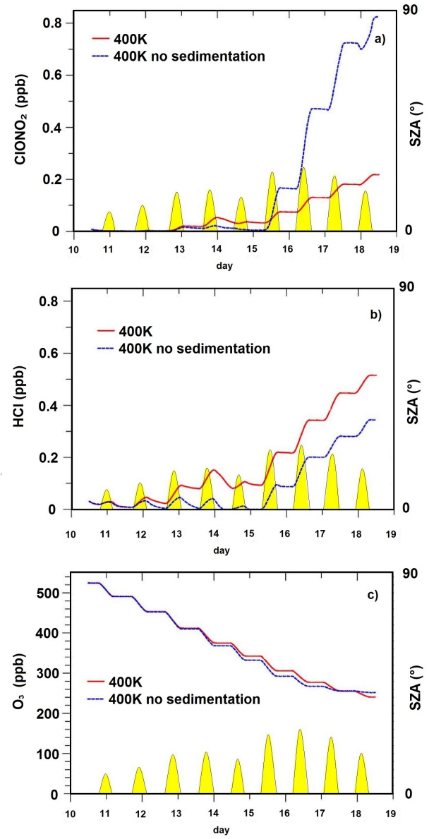
Figure 9. ClONO 2 (upper panel), HCl (middle) and O 3 (lower) evolution with (red line) and without (blue line) denitrification due to particle sedimentation.
