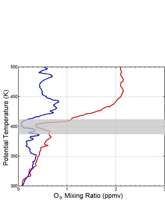
Figure 2. \text{O}_3 measurements from the in-situ ozonesonde (red line) on 10 Sept 2008, and on 20 Sept 2008 (blue line), vs potential temperature. The grey area highlights the air layer which returned over the Ross Sea less than 300 km from McMurdo.
