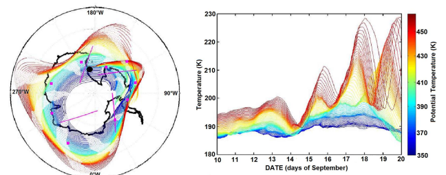
Figure 3. Left panel, air mass trajectories originating from McMurdo (black dot) and run 10 days forward, colour coded according to potential temperature. Solid coloured lines indicate sunlit legs, dotted lines indicate legs in darkness. Purple lines specify intersections with CALIOP footprint. Purple dots indicate where MLS data ( \text{O}_3 , \text{HNO}_3 or \text{HCl} ) were available. Right panel, temperature values along the trajectories, again colour coded in term of potential temperature.
