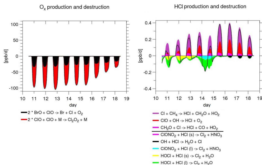
Figure 7. Left panel: O_3 depletion rates due to ClO - BrO (black) and ClO - ClO (red) catalytic cycles. Right panel: HCl production and depletion rates due to the set of reactions listed at the bottom of the panel. Simulation have been carried out on the 400 K isentropic level.
