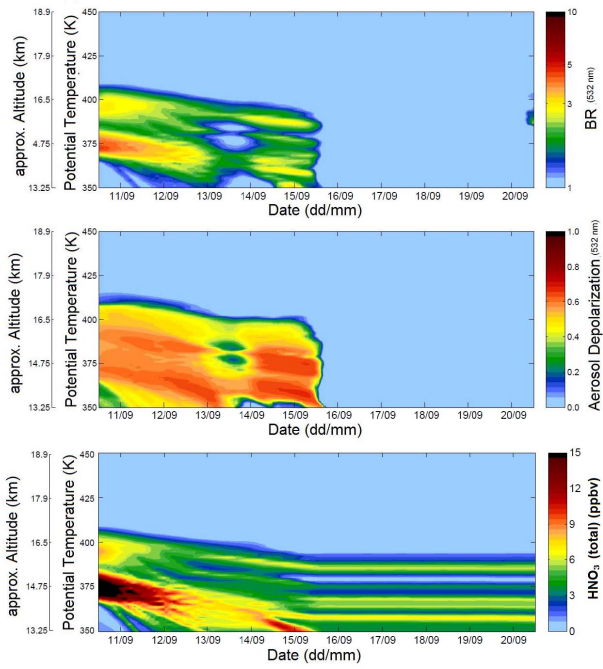
Figure 5. Profiles of Backscatter Ratio (upper panel), Aerosol Depolarization Ratio (middle panel) and total \text{HNO}_3 (lower panel) starting from the observations taken on September 10, 2008, and evolving according to the microphysical model.
