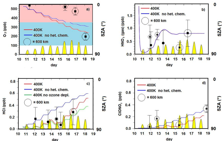
Figure 6. MLS (squares) and MIPAS (stars) observations and model results with (red line) and without (blue line) heterogeneous chemistry. a) (upper left panel) O_3 the colored areas highlight the range of variability of O_3 values observed by the balloonborne ozonesonde in the 400 \pm 10 K air layer which returned over the Ross Sea less than 300 km from McMurdo: Red for the first flight, Blue for the second flight; b) (upper right) HNO_3 ; c) (lower left) HCl ; d) (lower right) ClONO_2 . The radius of the circles surrounding the data points represents the match radius. Yellow areas indicate sunlit parts of the trajectory, the corresponding solar zenith angle (SZA) is reported on the right vertical axis.
