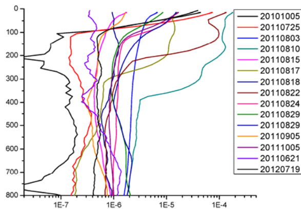
Figure: Aerosol backscatter coefficient (in \text{m}^{-1} \text{sr}^{-1} ) versus height (in m) below cloud base. Cloud base is always precisely detected with the multiple scattering (MS) channel (the outer FOV channel). The MS channel only receives a strong signal in case of cloud drops ( 50\text{--}500 \text{ cm}^{-3} ) and thus clearly identifies the cloud base. 15 backscatter profiles out of the used 26 backscatter profiles are shown.
