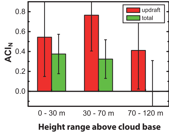
Fig. 5. ACI_N for updraft periods only (red, 13 cases) and when vertical wind information is not taken into account in the lidar data analysis and ACI_N retrieval (green, 26 cases). Error bars show the overall variability caused by atmospheric variability and retrieval uncertainties.
