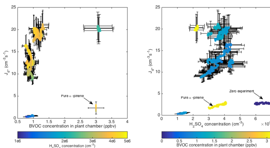
Figure 4. (a) Particle formation rates ( J ) as function of BVOC concentration, and marker colours indicate the corresponding \text{H}_2\text{SO}_4 concentrations in log scales. (b) Particle formation rates ( J ) as function of \text{H}_2\text{SO}_4 concentrations. Marker colours indicate the corresponding BVOC concentration from the inlet flow. Square markers show data from alpha-pinene experiments; star markers show a zero experiment with no BVOC added.
