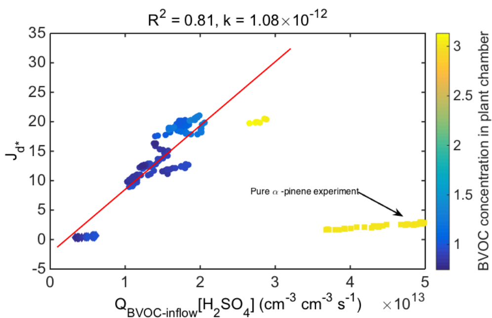
Figure 5. Particle formation rates ( J ) as function of the product of BVOC inflow and sulphuric acid concentration. Marker colours indicate the corresponding monoterpene concentration from the inlet flow of JPAC reaction chamber. The pure \alpha -pinene experiments indicated in the figure were not included in the linear fit.
