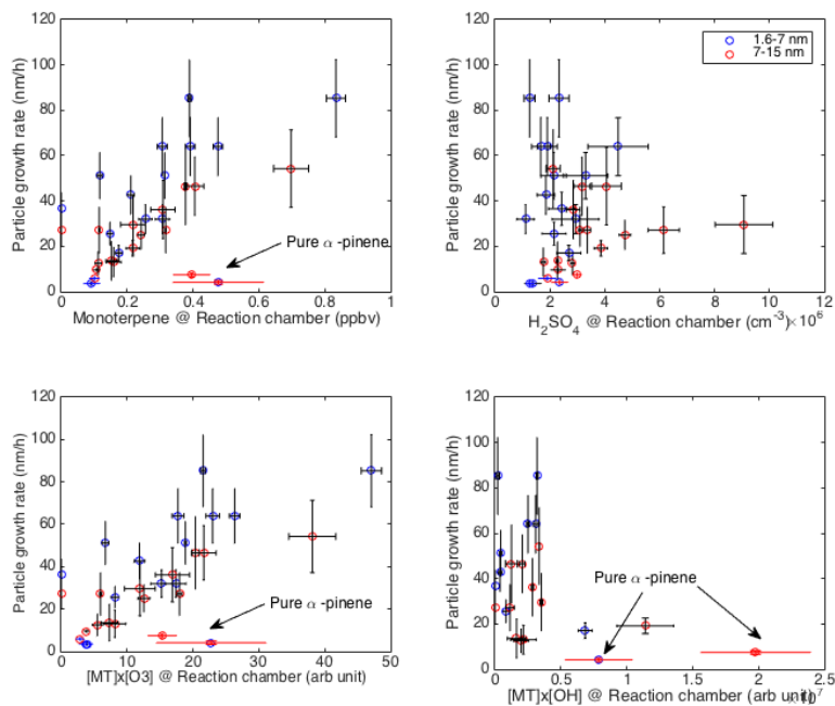
Figure 6. Particle growth rates (GR) at the beginning of the particle formation burst as function of (a) monoterpene concentrations in the JPAC reaction chamber, (b) H_2SO_4 concentrations in the JPAC reaction chamber. (c) Proxy concentrations of oxidation products of monoterpenes by O_3 in the JPAC reaction chamber (d) proxy concentrations of oxidation products of monoterpenes by OH in the JPAC reaction chamber. Red squares are growth rates of particles ranging from 1.6–7 nm, and blues markers indicates growth rates of particles with diameter of 7–15 nm.
